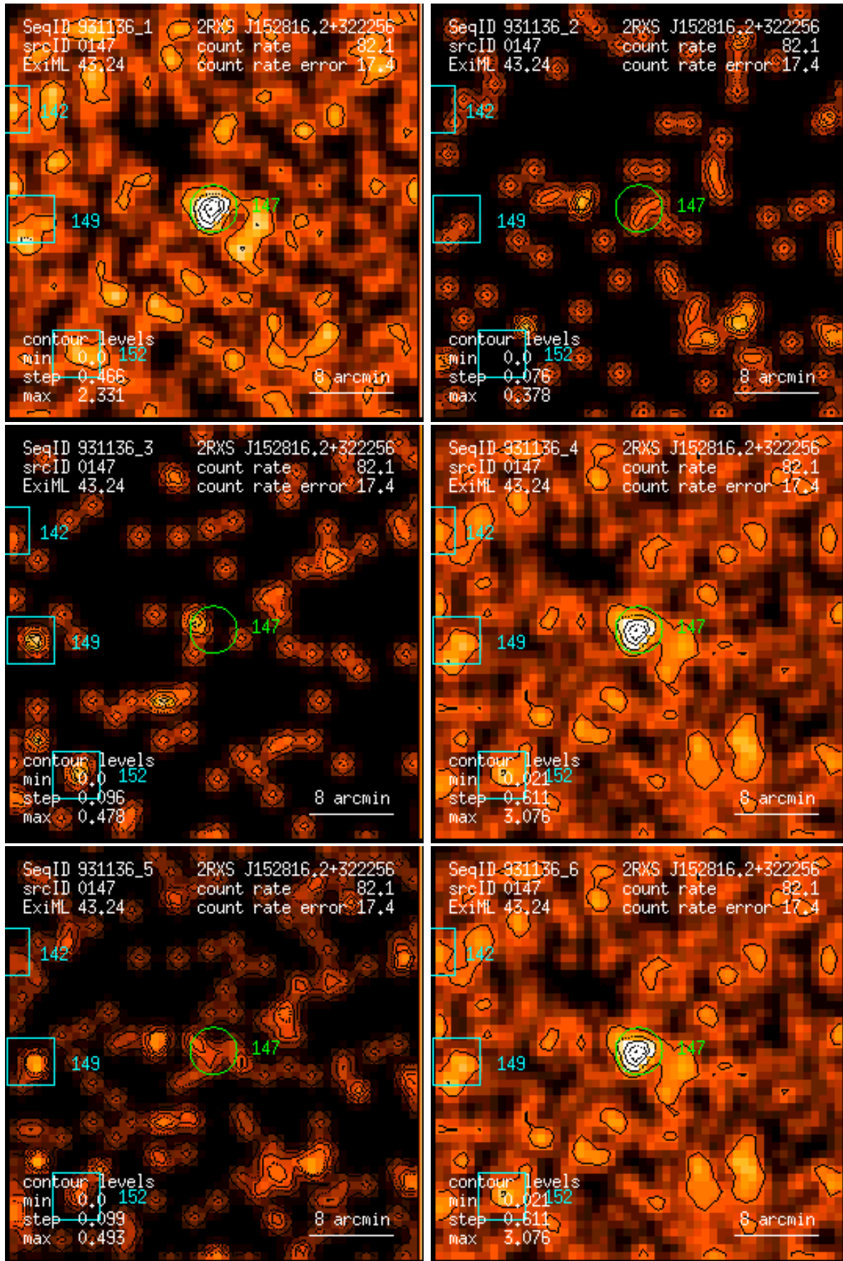
Figure 147: RASS 931136: detection 0147: band rate images, Gaussian filter: (1) PSPC channels 11 – 41, (2) 52 – 90, (3) 91 – 201, (4) 11 – 235, (5) 52 – 201, (6) 11 – 201. Broad band rates in counts/ks. Band rate contour levels in counts/ks/arcmin 2 .
