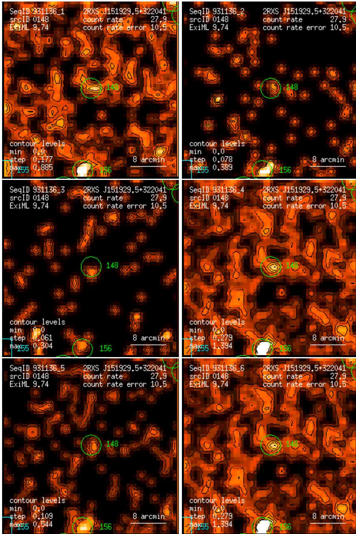
Figure 148: RASS 931136: detection 0148: band rate images, Gaussian filter: (1) PSPC channels 11 – 41, (2) 52 – 90, (3) 91 – 201, (4) 11 – 235, (5) 52 – 201, (6) 11 – 201. Broad band rates in counts/ks. Band rate contour levels in counts/ks/arcmin 2 .
