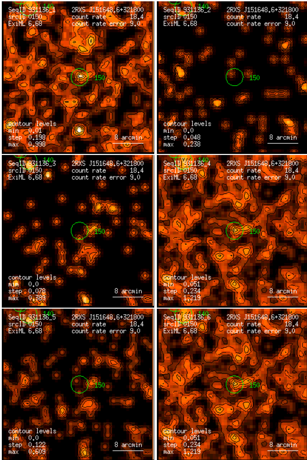
Figure 150: RASS 931136: detection 0150: band rate images, Gaussian filter: (1) PSPC channels 11 – 41, (2) 52 – 90, (3) 91 – 201, (4) 11 – 235, (5) 52 – 201, (6) 11 – 201. Broad band rates in counts/ks. Band rate contour levels in counts/ks/arcmin 2 .
