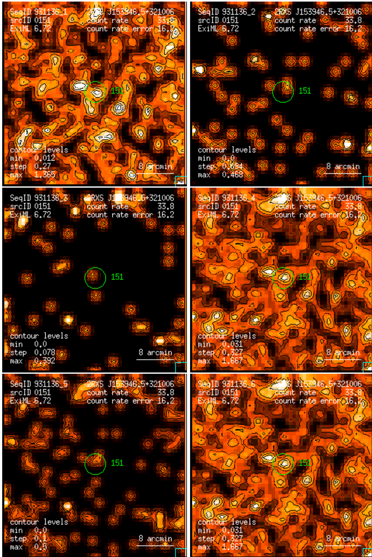
Figure 151: RASS 931136: detection 0151: band rate images, Gaussian filter: (1) PSPC channels 11 – 41, (2) 52 – 90, (3) 91 – 201, (4) 11 – 235, (5) 52 – 201, (6) 11 – 201. Broad band rates in counts/ks. Band rate contour levels in counts/ks/arcmin 2 .
