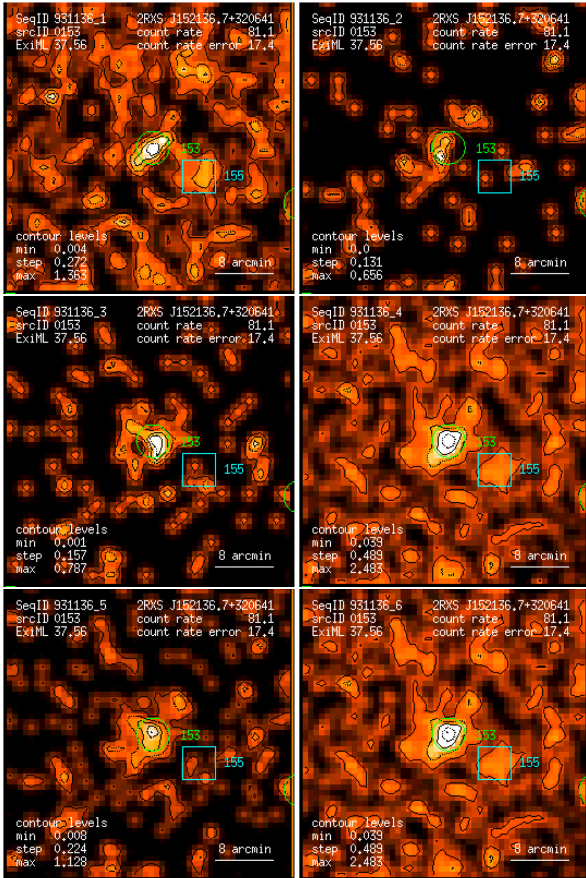
Figure 153: RASS 931136: detection 0153: band rate images, Gaussian filter: (1) PSPC channels 11 – 41, (2) 52 – 90, (3) 91 – 201, (4) 11 – 235, (5) 52 – 201, (6) 11 – 201. Broad band rates in counts/ks. Band rate contour levels in counts/ks/arcmin 2 .
