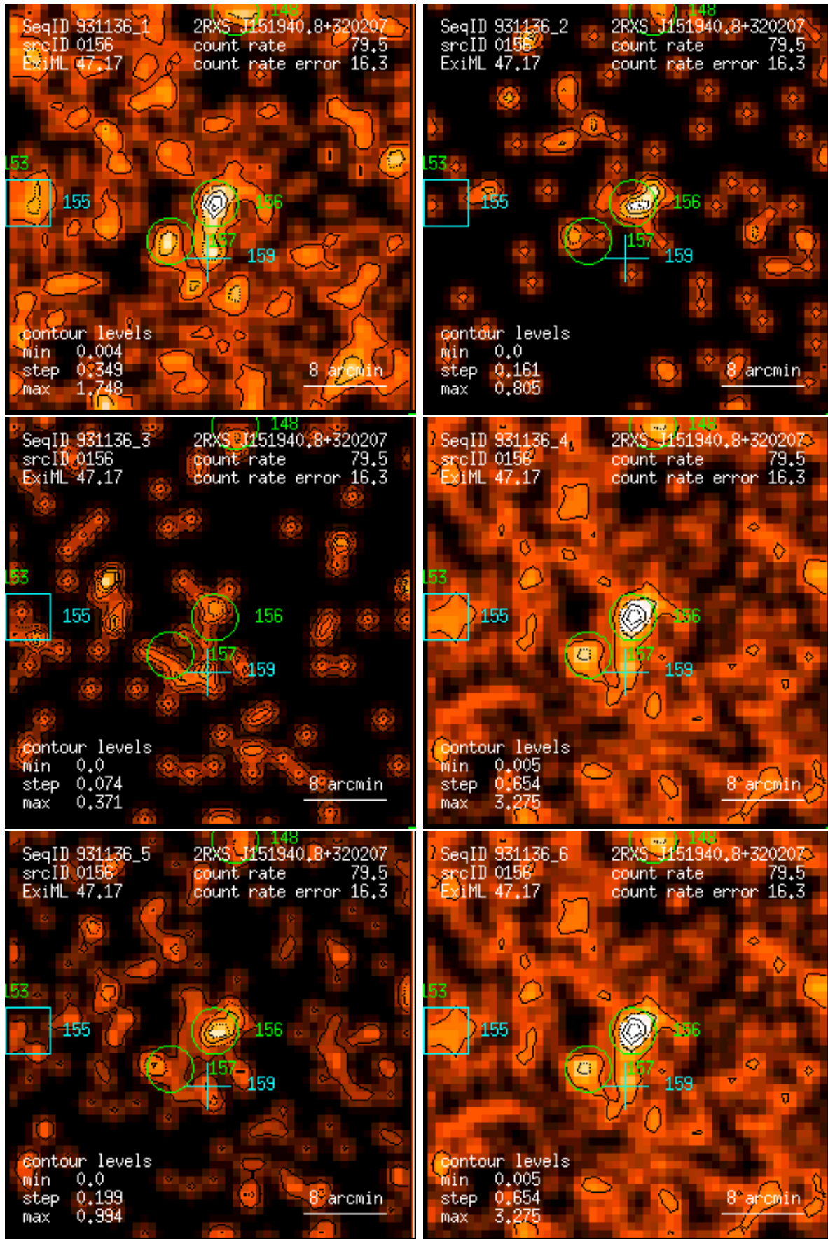
Figure 156: RASS 931136: detection 0156: band rate images, Gaussian filter: (1) PSPC channels 11 – 41, (2) 52 – 90, (3) 91 – 201, (4) 11 – 235, (5) 52 – 201, (6) 11 – 201. Broad band rates in counts/ks. Band rate contour levels in counts/ks/arcmin 2 .
