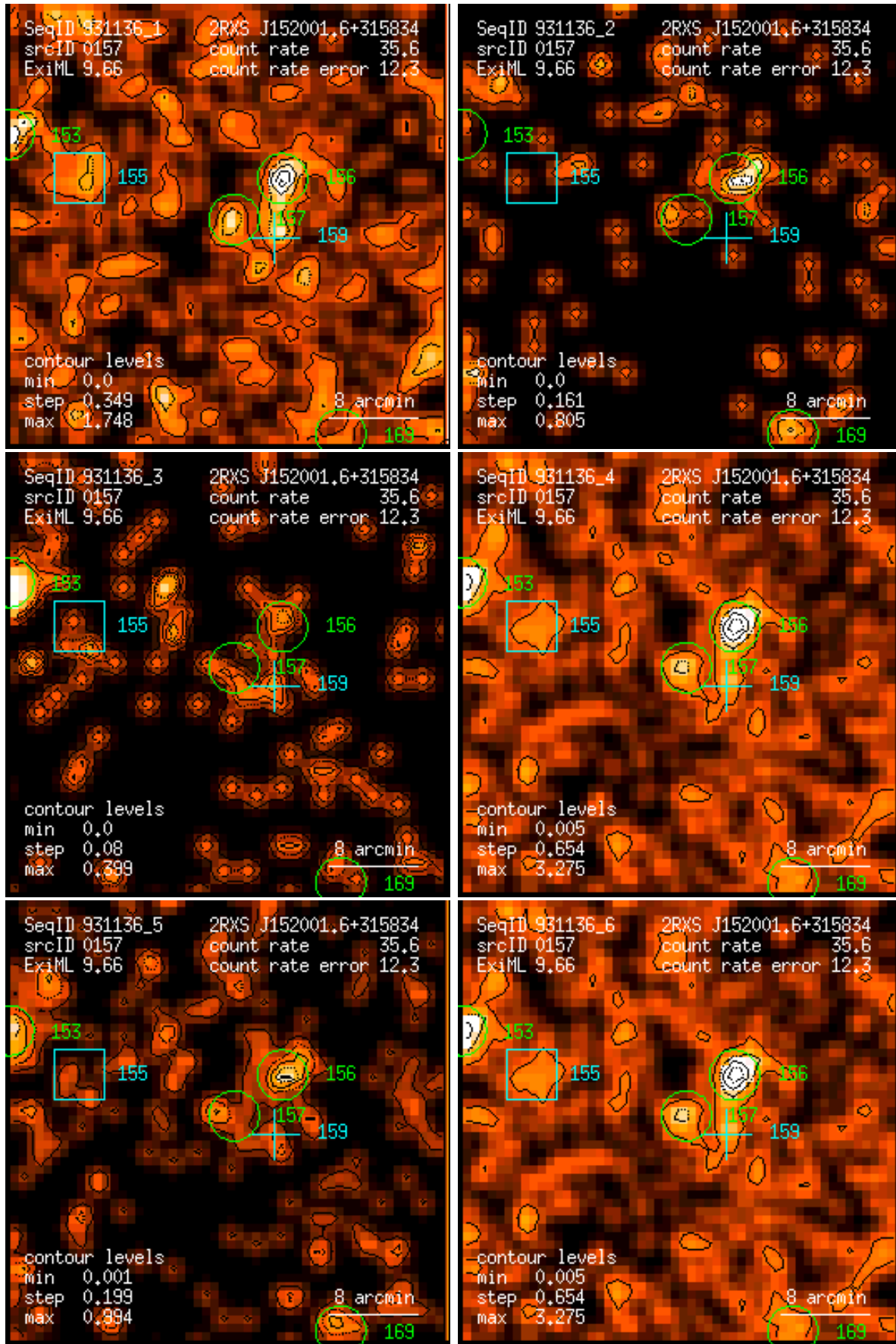
Figure 157: RASS 931136: detection 0157: band rate images, Gaussian filter: (1) PSPC channels 11 – 41, (2) 52 – 90, (3) 91 – 201, (4) 11 – 235, (5) 52 – 201, (6) 11 – 201. Broad band rates in counts/ks. Band rate contour levels in counts/ks/arcmin 2 .
