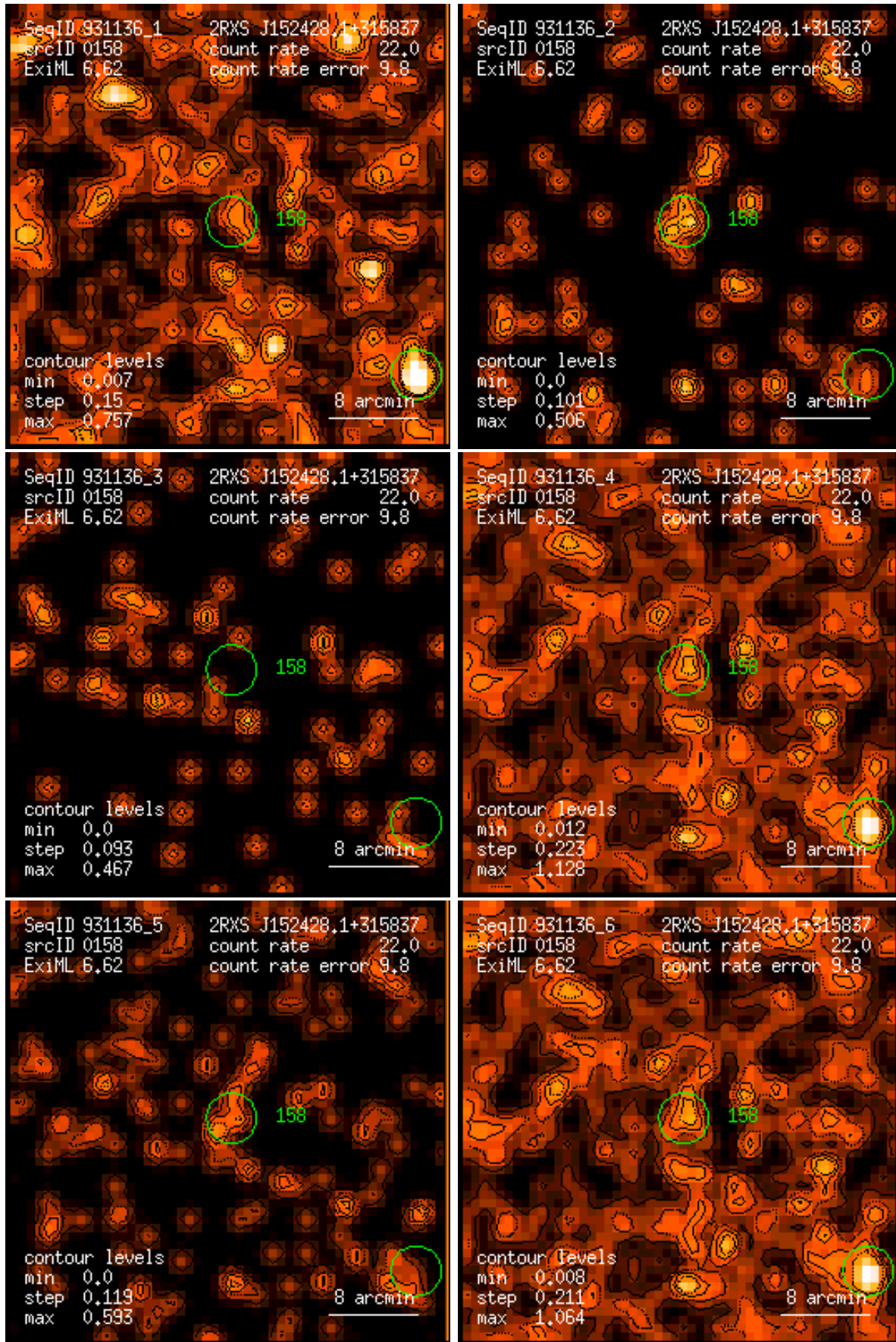
Figure 158: RASS 931136: detection 0158: band rate images, Gaussian filter: (1) PSPC channels 11 – 41, (2) 52 – 90, (3) 91 – 201, (4) 11 – 235, (5) 52 – 201, (6) 11 – 201. Broad band rates in counts/ks. Band rate contour levels in counts/ks/arcmin 2 .
