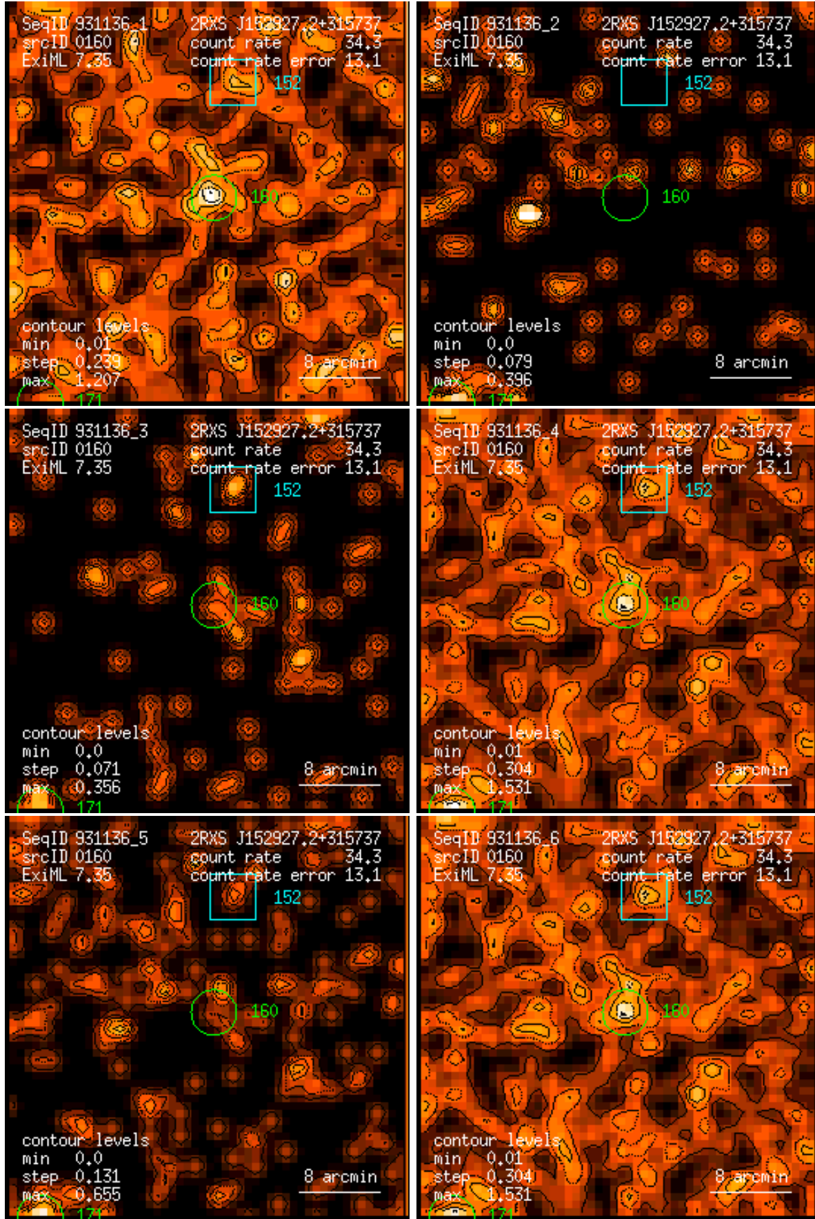
Figure 160: RASS 931136: detection 0160: band rate images, Gaussian filter: (1) PSPC channels 11 – 41, (2) 52 – 90, (3) 91 – 201, (4) 11 – 235, (5) 52 – 201, (6) 11 – 201. Broad band rates in counts/ks. Band rate contour levels in counts/ks/arcmin 2 .
