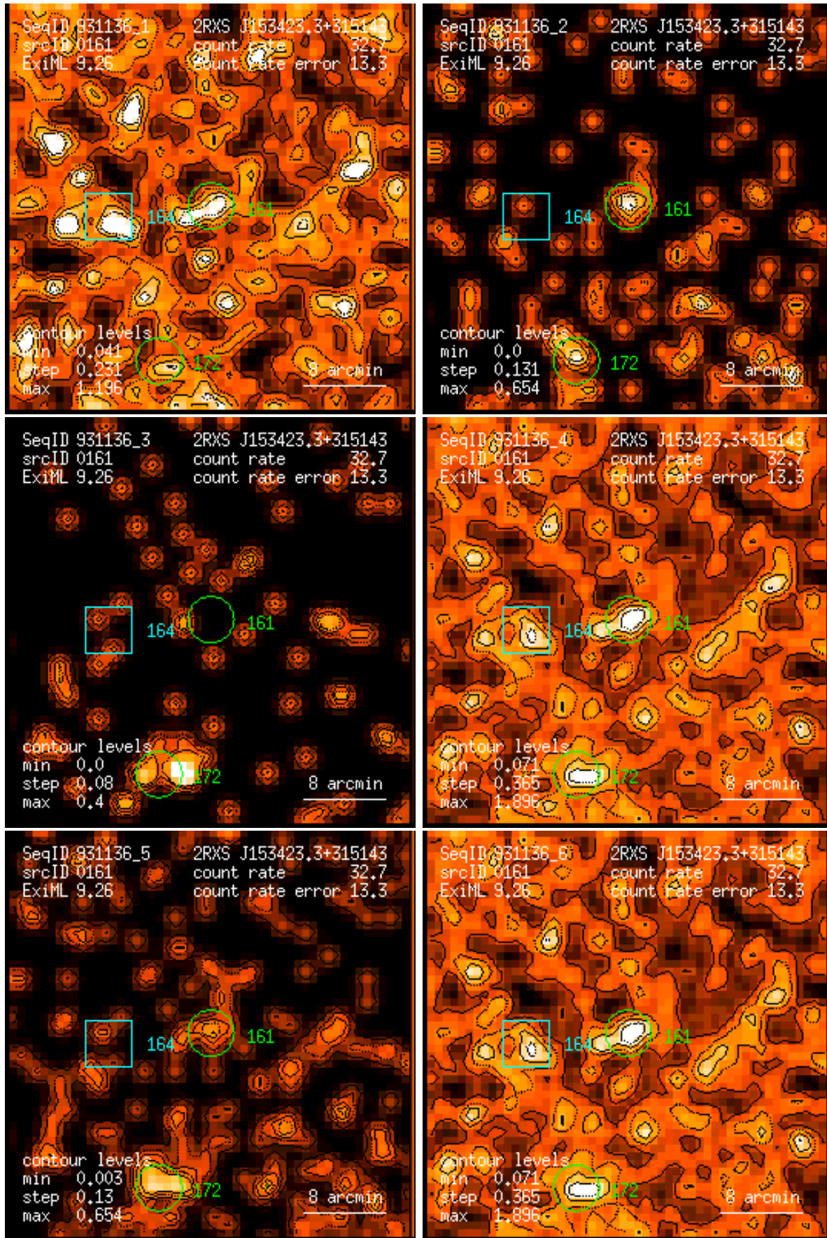
Figure 161: RASS 931136: detection 0161: band rate images, Gaussian filter: (1) PSPC channels 11 – 41, (2) 52 – 90, (3) 91 – 201, (4) 11 – 235, (5) 52 – 201, (6) 11 – 201. Broad band rates in counts/ks. Band rate contour levels in counts/ks/arcmin 2 .
