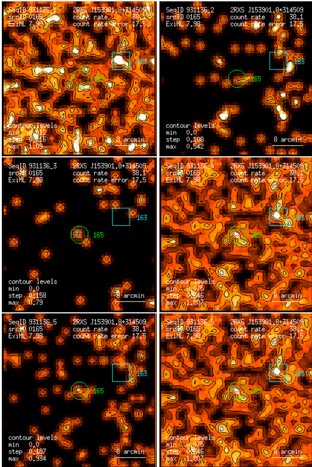
Figure 165: RASS 931136: detection 0165: band rate images, Gaussian filter: (1) PSPC channels 11 – 41, (2) 52 – 90, (3) 91 – 201, (4) 11 – 235, (5) 52 – 201, (6) 11 – 201. Broad band rates in counts/ks. Band rate contour levels in counts/ks/arcmin 2 .
