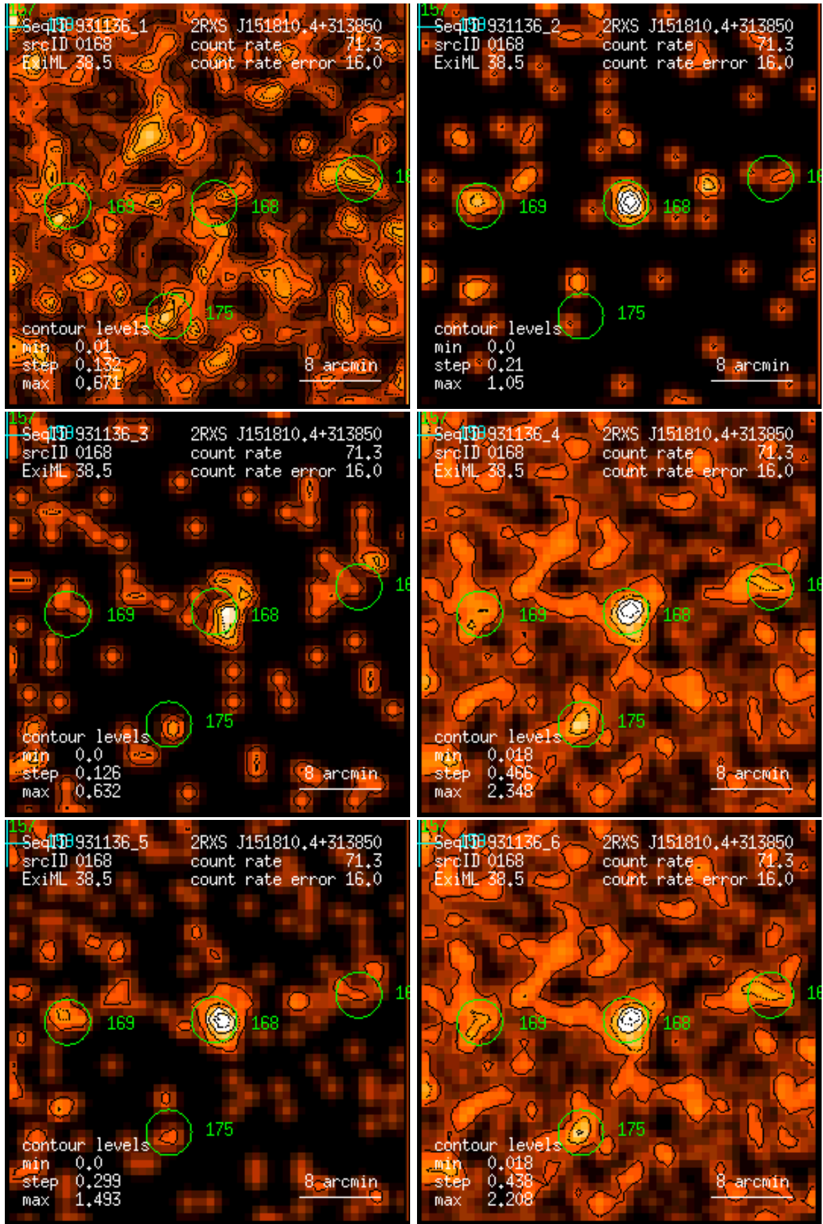
Figure 168: RASS 931136: detection 0168: band rate images, Gaussian filter: (1) PSPC channels 11 – 41, (2) 52 – 90, (3) 91 – 201, (4) 11 – 235, (5) 52 – 201, (6) 11 – 201. Broad band rates in counts/ks. Band rate contour levels in counts/ks/arcmin 2 .
