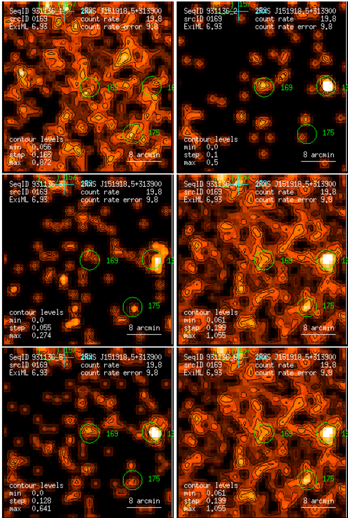
Figure 169: RASS 931136: detection 0169: band rate images, Gaussian filter: (1) PSPC channels 11 – 41, (2) 52 – 90, (3) 91 – 201, (4) 11 – 235, (5) 52 – 201, (6) 11 – 201. Broad band rates in counts/ks. Band rate contour levels in counts/ks/arcmin 2 .
