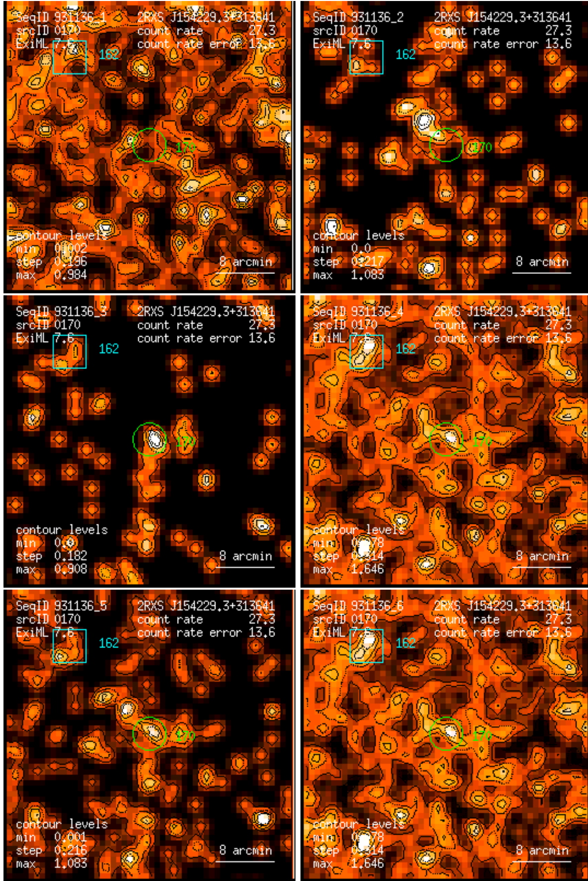
Figure 170: RASS 931136: detection 0170: band rate images, Gaussian filter: (1) PSPC channels 11 – 41, (2) 52 – 90, (3) 91 – 201, (4) 11 – 235, (5) 52 – 201, (6) 11 – 201. Broad band rates in counts/ks. Band rate contour levels in counts/ks/arcmin 2 .
