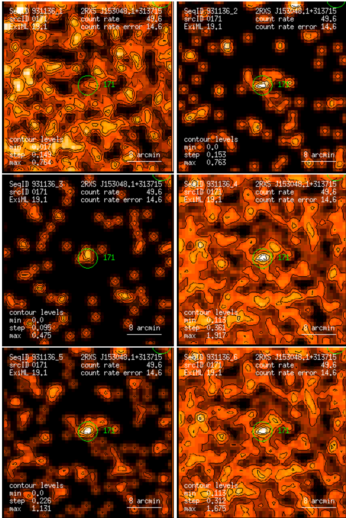
Figure 171: RASS 931136: detection 0171: band rate images, Gaussian filter: (1) PSPC channels 11 – 41, (2) 52 – 90, (3) 91 – 201, (4) 11 – 235, (5) 52 – 201, (6) 11 – 201. Broad band rates in counts/ks. Band rate contour levels in counts/ks/arcmin 2 .
