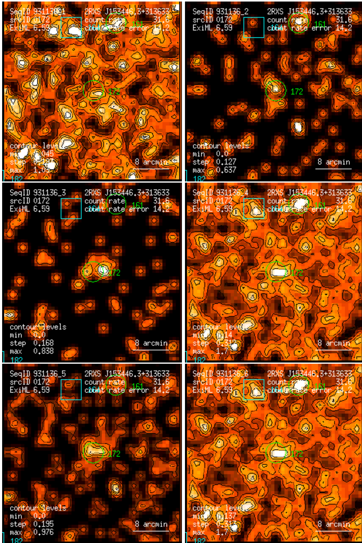
Figure 172: RASS 931136: detection 0172: band rate images, Gaussian filter: (1) PSPC channels 11 – 41, (2) 52 – 90, (3) 91 – 201, (4) 11 – 235, (5) 52 – 201, (6) 11 – 201. Broad band rates in counts/ks. Band rate contour levels in counts/ks/arcmin 2 .
