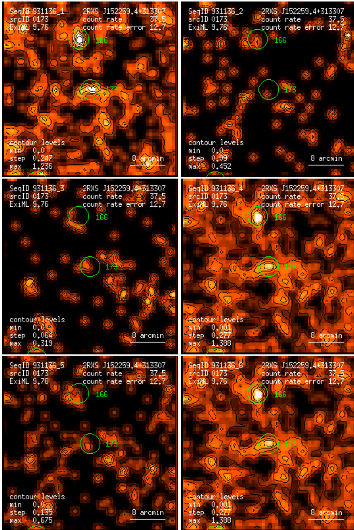
Figure 173: RASS 931136: detection 0173: band rate images, Gaussian filter: (1) PSPC channels 11 – 41, (2) 52 – 90, (3) 91 – 201, (4) 11 – 235, (5) 52 – 201, (6) 11 – 201. Broad band rates in counts/ks. Band rate contour levels in counts/ks/arcmin 2 .
