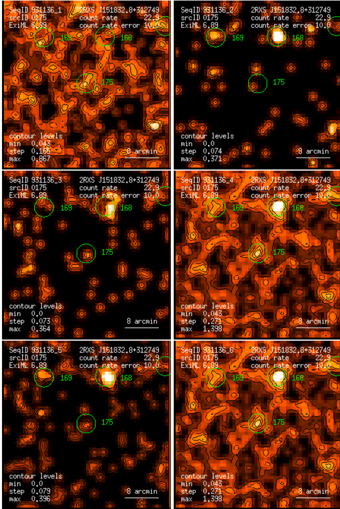
Figure 175: RASS 931136: detection 0175: band rate images, Gaussian filter: (1) PSPC channels 11 – 41, (2) 52 – 90, (3) 91 – 201, (4) 11 – 235, (5) 52 – 201, (6) 11 – 201. Broad band rates in counts/ks. Band rate contour levels in counts/ks/arcmin 2 .
