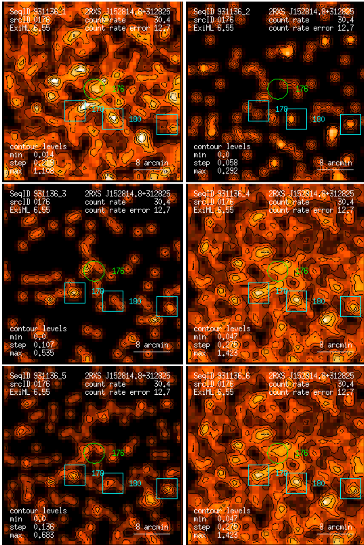
Figure 176: RASS 931136: detection 0176: band rate images, Gaussian filter: (1) PSPC channels 11 – 41, (2) 52 – 90, (3) 91 – 201, (4) 11 – 235, (5) 52 – 201, (6) 11 – 201. Broad band rates in counts/ks. Band rate contour levels in counts/ks/arcmin 2 .
