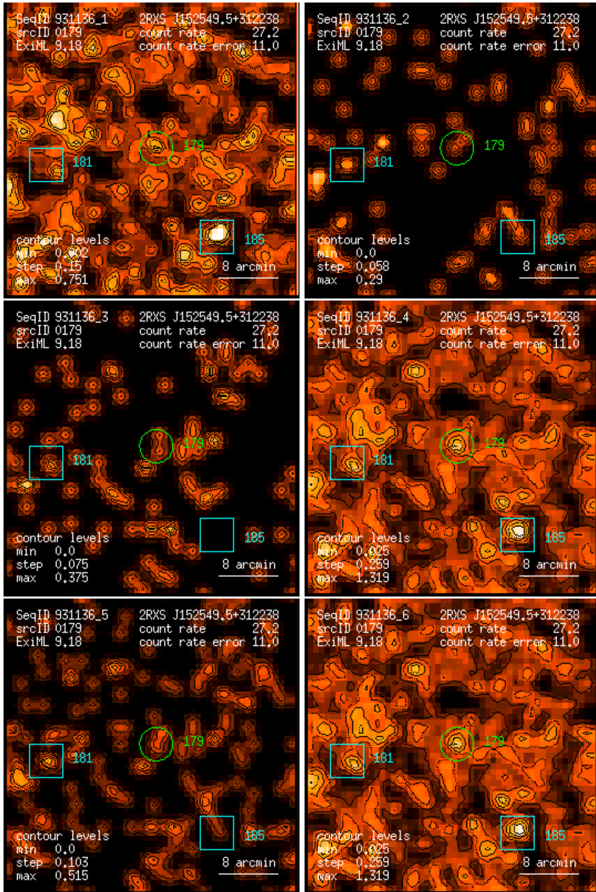
Figure 179: RASS 931136: detection 0179: band rate images, Gaussian filter: (1) PSPC channels 11 – 41, (2) 52 – 90, (3) 91 – 201, (4) 11 – 235, (5) 52 – 201, (6) 11 – 201. Broad band rates in counts/ks. Band rate contour levels in counts/ks/arcmin 2 .
