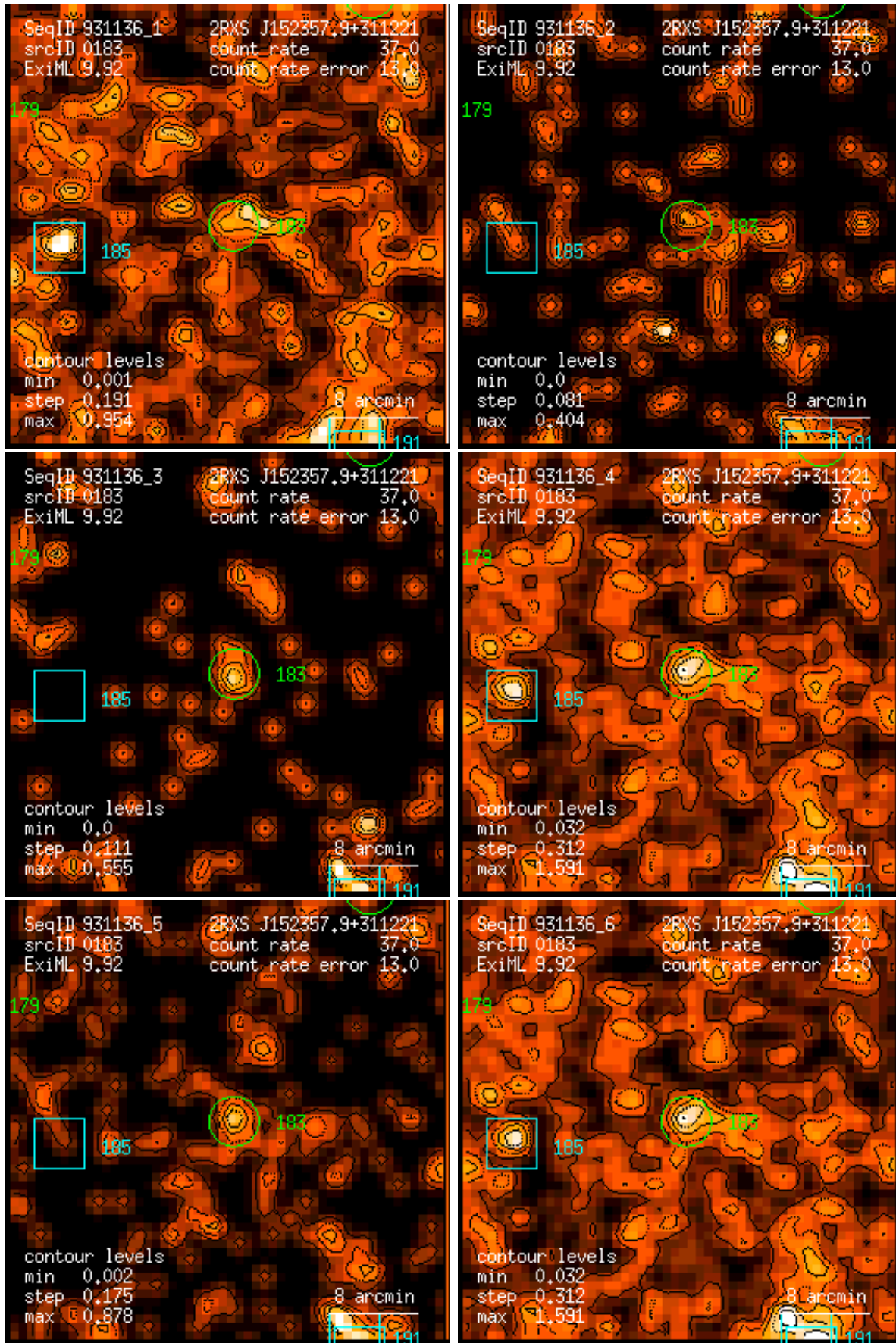
Figure 183: RASS 931136: detection 0183: band rate images, Gaussian filter: (1) PSPC channels 11 – 41, (2) 52 – 90, (3) 91 – 201, (4) 11 – 235, (5) 52 – 201, (6) 11 – 201. Broad band rates in counts/ks. Band rate contour levels in counts/ks/arcmin 2 .
