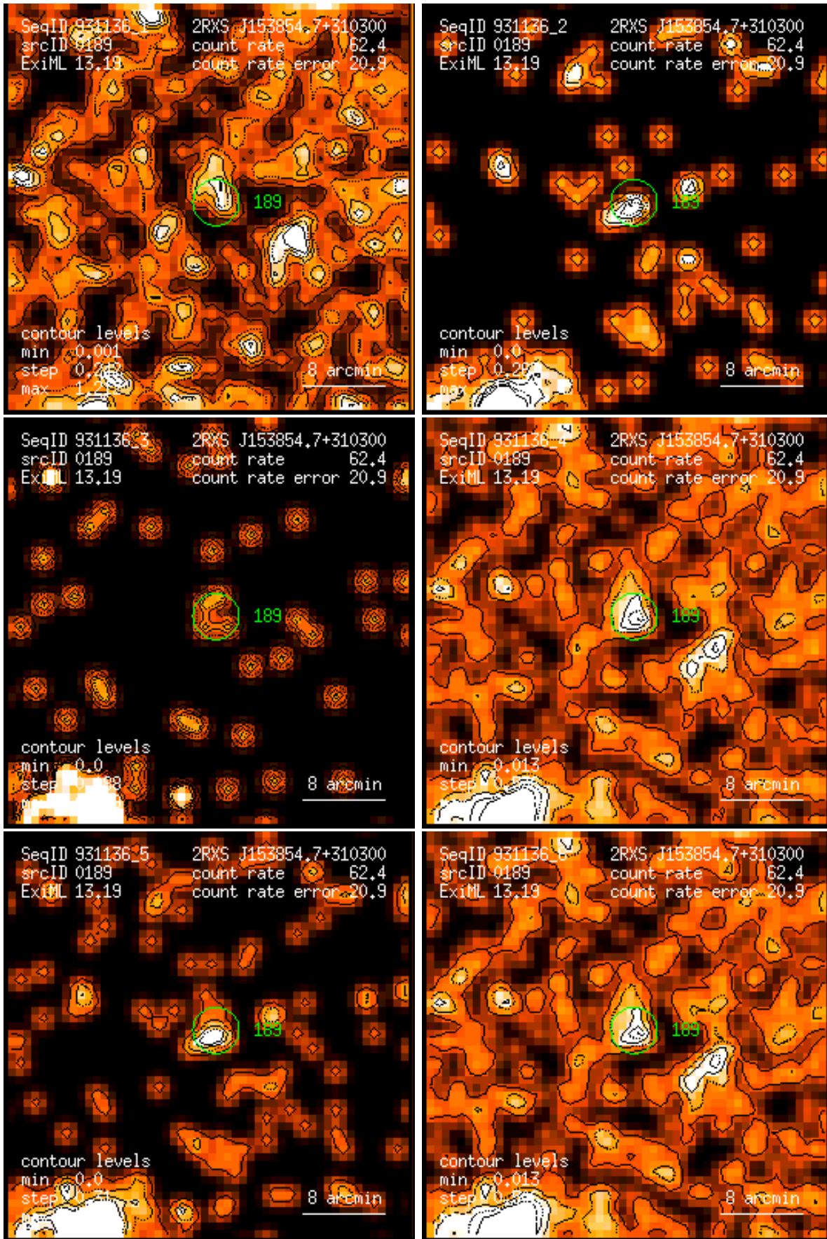
Figure 189: RASS 931136: detection 0189: band rate images, Gaussian filter: (1) PSPC channels 11 – 41, (2) 52 – 90, (3) 91 – 201, (4) 11 – 235, (5) 52 – 201, (6) 11 – 201. Broad band rates in counts/ks. Band rate contour levels in counts/ks/arcmin 2 .
