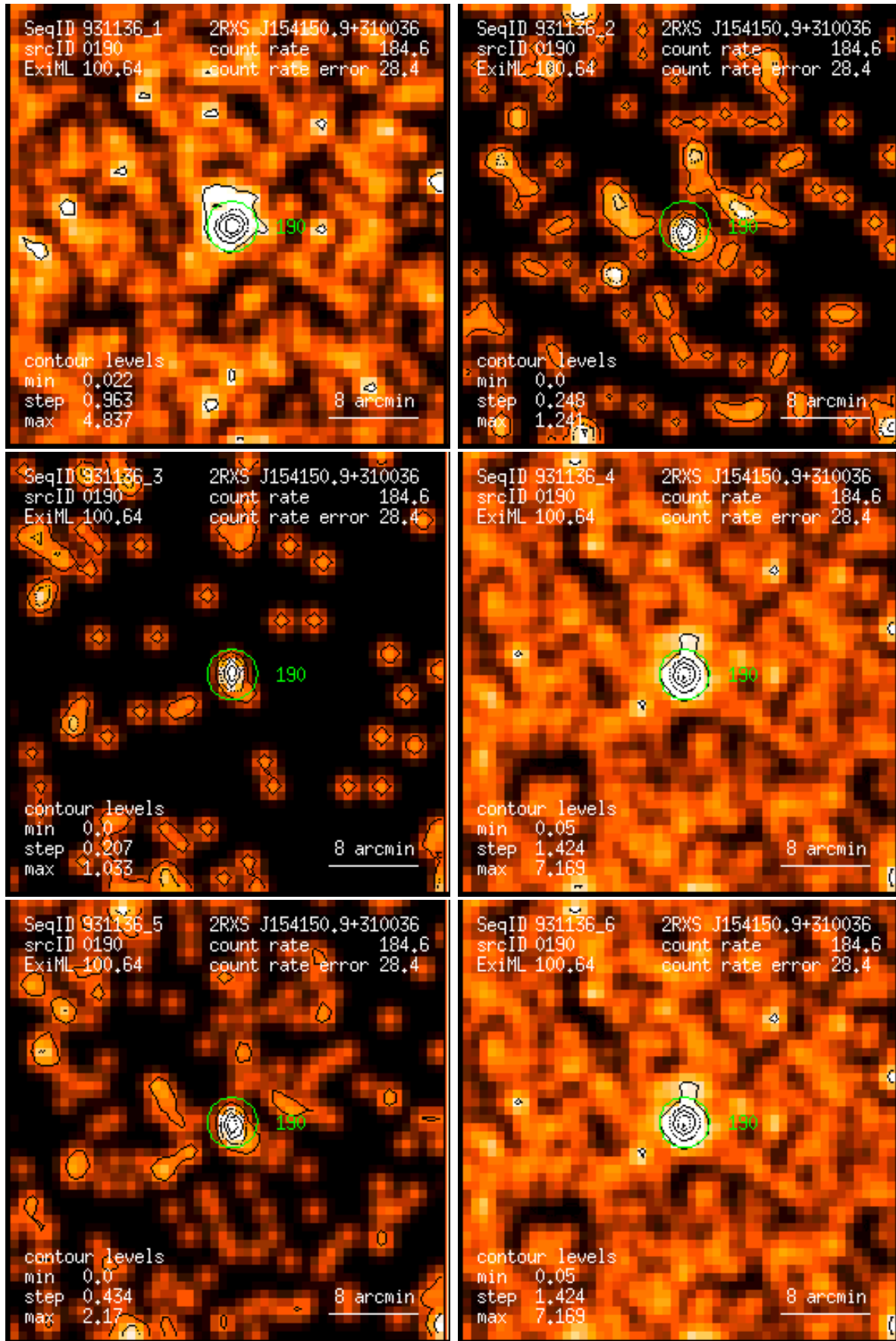
Figure 190: RASS 931136: detection 0190: band rate images, Gaussian filter: (1) PSPC channels 11 – 41, (2) 52 – 90, (3) 91 – 201, (4) 11 – 235, (5) 52 – 201, (6) 11 – 201. Broad band rates in counts/ks. Band rate contour levels in counts/ks/arcmin 2 .
