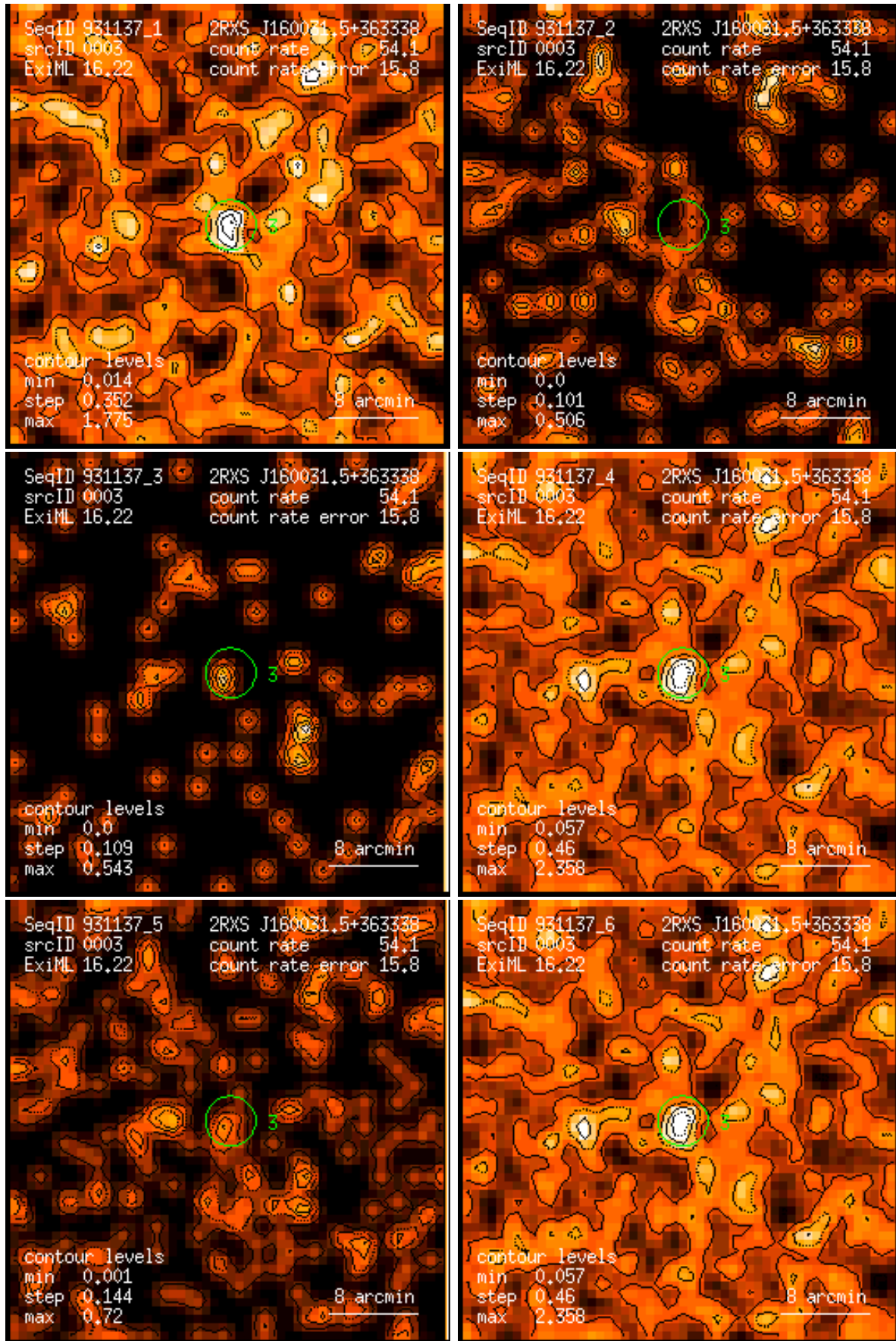
Figure 3: RASS 931137: detection 0003: band rate images, Gaussian filter: (1) PSPC channels 11 – 41, (2) 52 – 90, (3) 91 – 201, (4) 11 – 235, (5) 52 – 201, (6) 11 – 201. Broad band rates in counts/ks. Band rate contour levels in counts/ks/arcmin 2 .
