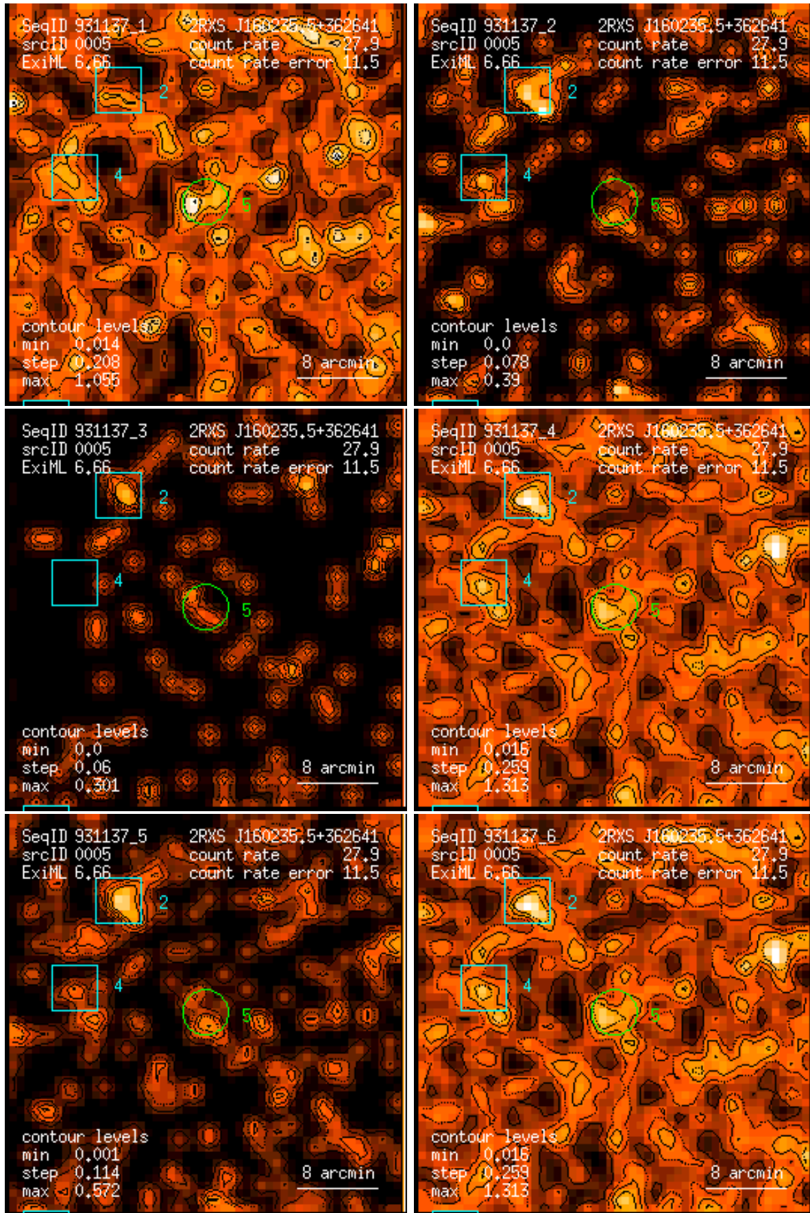
Figure 5: RASS 931137: detection 0005: band rate images, Gaussian filter: (1) PSPC channels 11 – 41, (2) 52 – 90, (3) 91 – 201, (4) 11 – 235, (5) 52 – 201, (6) 11 – 201. Broad band rates in counts/ks. Band rate contour levels in counts/ks/arcmin 2 .
