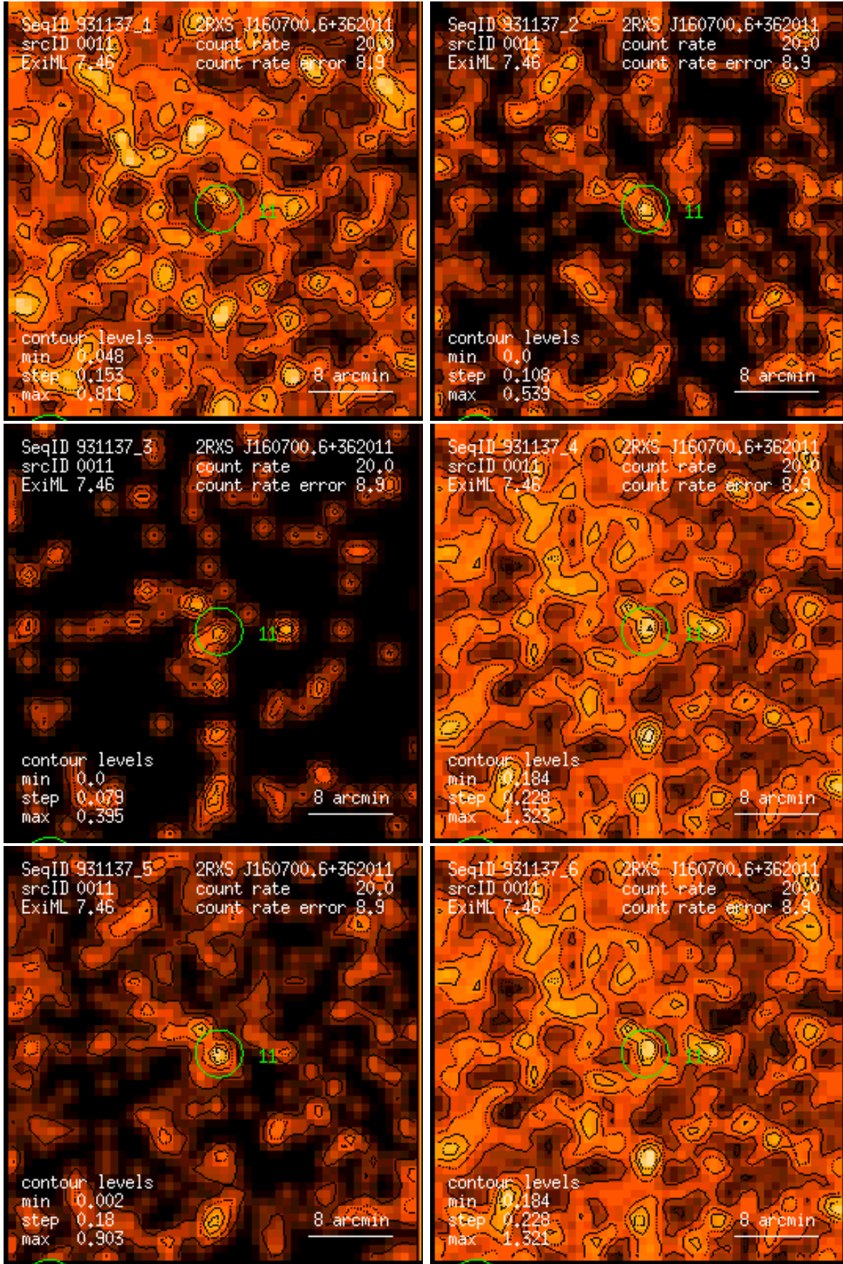
Figure 11: RASS 931137: detection 0011: band rate images, Gaussian filter: (1) PSPC channels 11 – 41, (2) 52 – 90, (3) 91 – 201, (4) 11 – 235, (5) 52 – 201, (6) 11 – 201. Broad band rates in counts/ks. Band rate contour levels in counts/ks/arcmin 2 .
