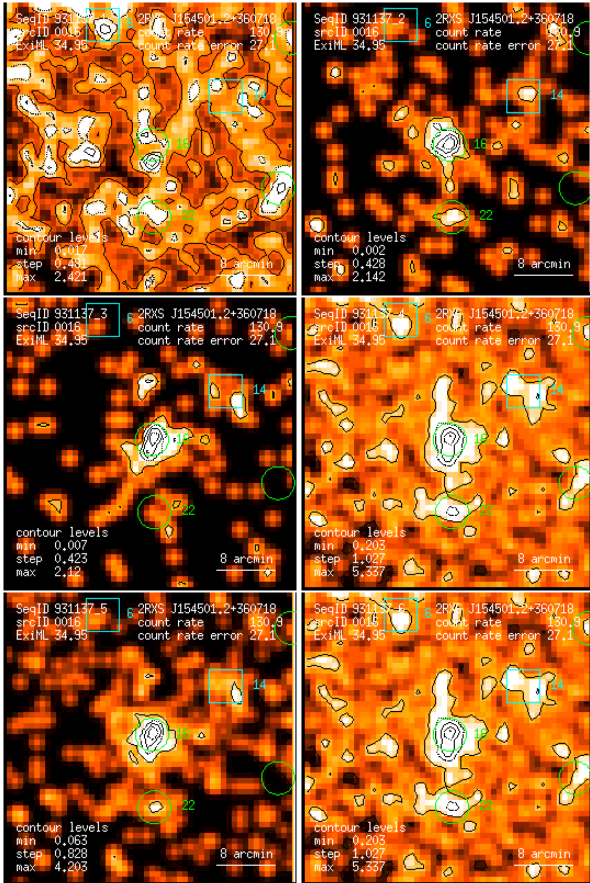
Figure 16: RASS 931137: detection 0016: band rate images, Gaussian filter: (1) PSPC channels 11 – 41, (2) 52 – 90, (3) 91 – 201, (4) 11 – 235, (5) 52 – 201, (6) 11 – 201. Broad band rates in counts/ks. Band rate contour levels in counts/ks/arcmin 2 .
