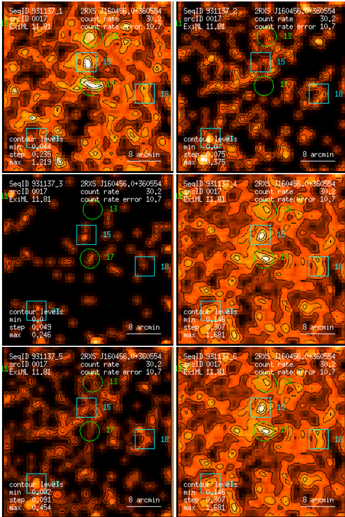
Figure 17: RASS 931137: detection 0017: band rate images, Gaussian filter: (1) PSPC channels 11 – 41, (2) 52 – 90, (3) 91 – 201, (4) 11 – 235, (5) 52 – 201, (6) 11 – 201. Broad band rates in counts/ks. Band rate contour levels in counts/ks/arcmin 2 .
