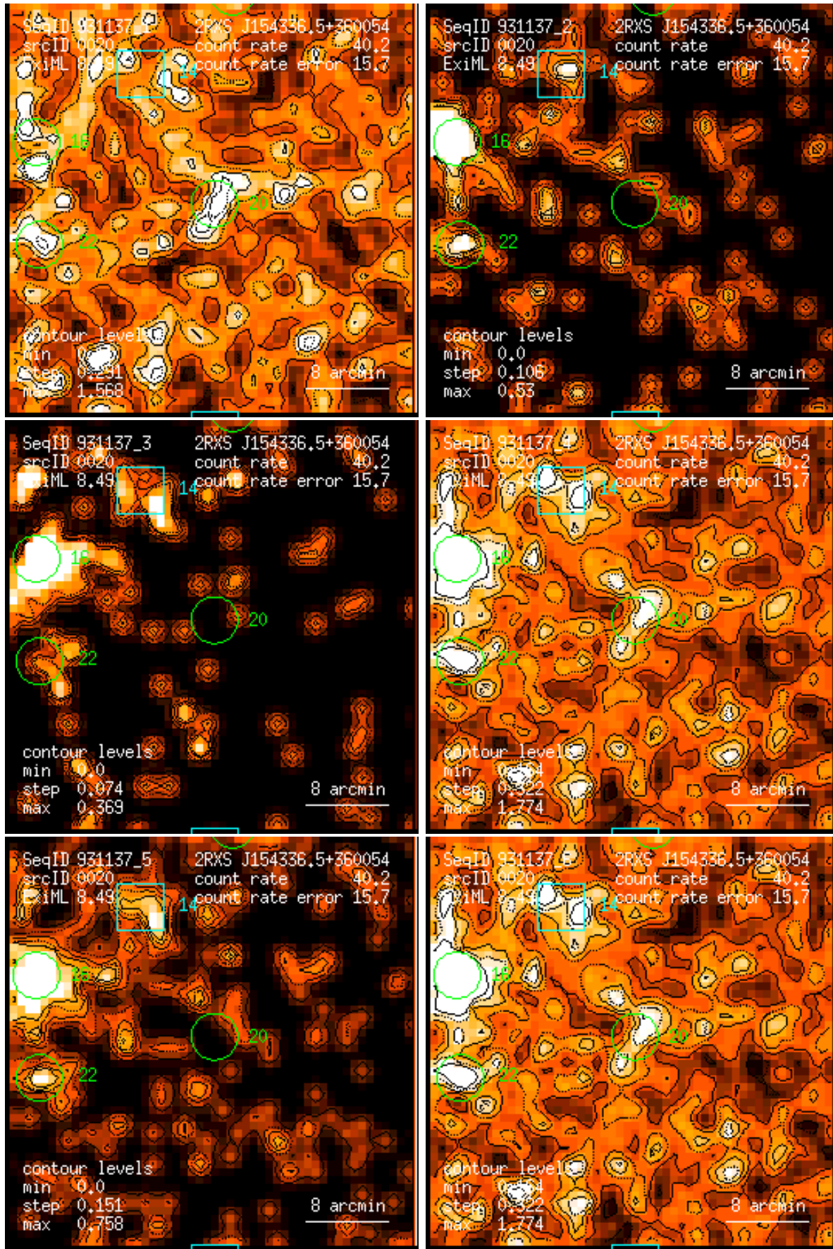
Figure 20: RASS 931137: detection 0020: band rate images, Gaussian filter: (1) PSPC channels 11 – 41, (2) 52 – 90, (3) 91 – 201, (4) 11 – 235, (5) 52 – 201, (6) 11 – 201. Broad band rates in counts/ks. Band rate contour levels in counts/ks/arcmin 2 .
