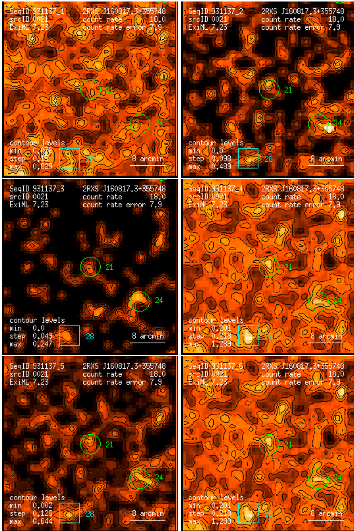
Figure 21: RASS 931137: detection 0021: band rate images, Gaussian filter: (1) PSPC channels 11 – 41, (2) 52 – 90, (3) 91 – 201, (4) 11 – 235, (5) 52 – 201, (6) 11 – 201. Broad band rates in counts/ks. Band rate contour levels in counts/ks/arcmin 2 .
