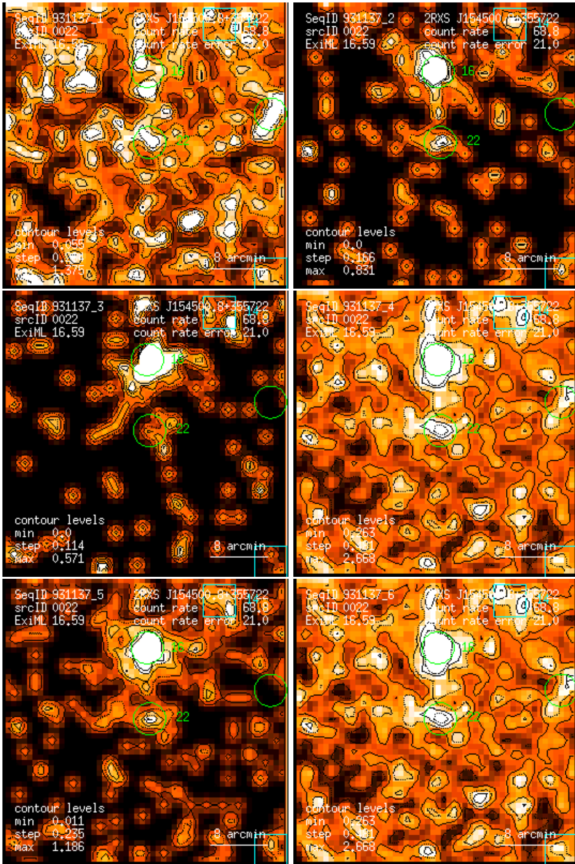
Figure 22: RASS 931137: detection 0022: band rate images, Gaussian filter: (1) PSPC channels 11 – 41, (2) 52 – 90, (3) 91 – 201, (4) 11 – 235, (5) 52 – 201, (6) 11 – 201. Broad band rates in counts/ks. Band rate contour levels in counts/ks/arcmin 2 .
