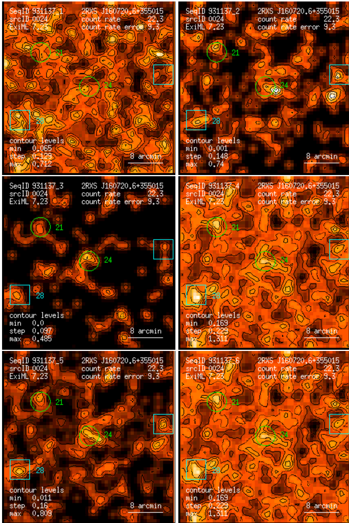
Figure 24: RASS 931137: detection 0024: band rate images, Gaussian filter: (1) PSPC channels 11 – 41, (2) 52 – 90, (3) 91 – 201, (4) 11 – 235, (5) 52 – 201, (6) 11 – 201. Broad band rates in counts/ks. Band rate contour levels in counts/ks/arcmin 2 .
