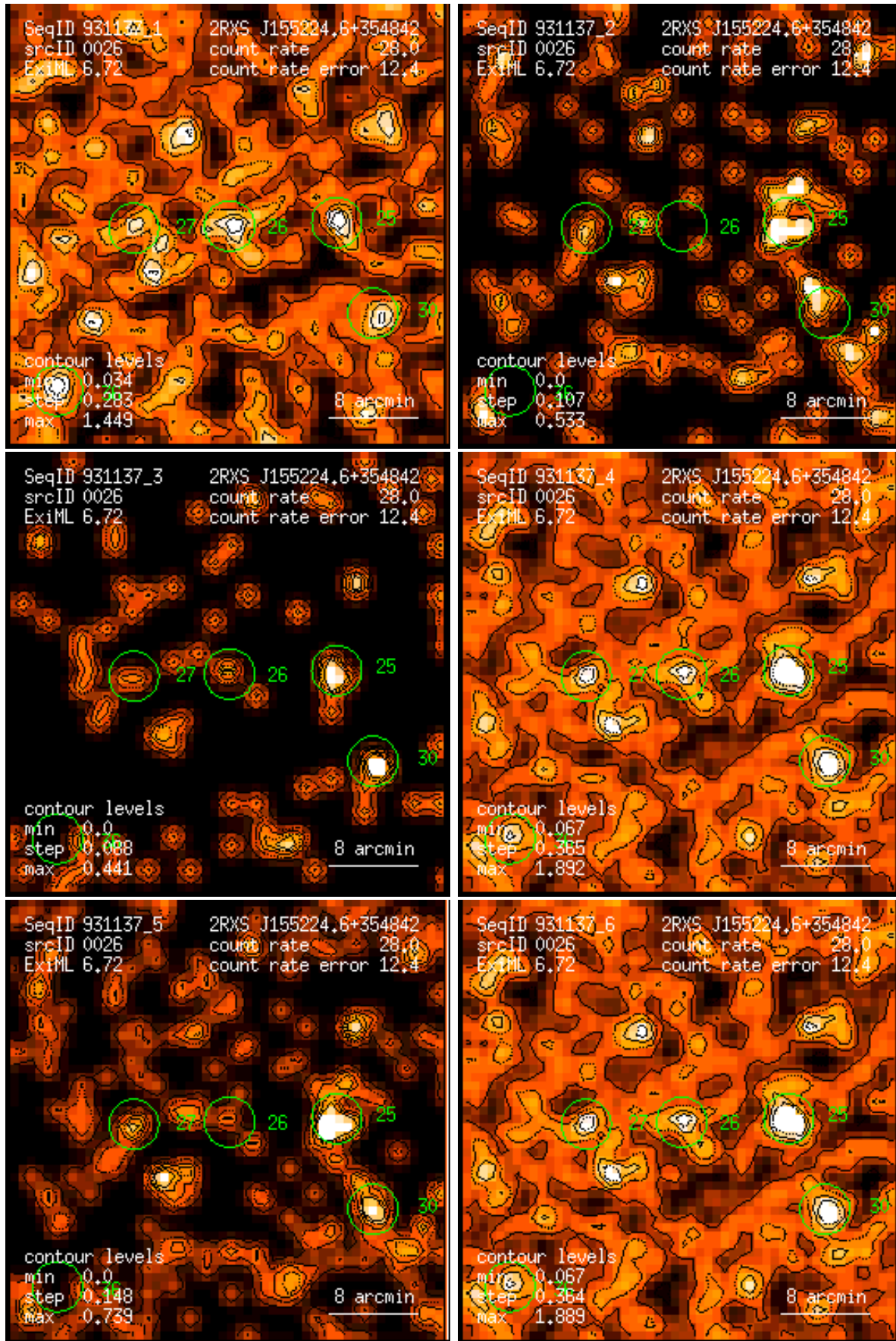
Figure 26: RASS 931137: detection 0026: band rate images, Gaussian filter: (1) PSPC channels 11 – 41, (2) 52 – 90, (3) 91 – 201, (4) 11 – 235, (5) 52 – 201, (6) 11 – 201. Broad band rates in counts/ks. Band rate contour levels in counts/ks/arcmin 2 .
