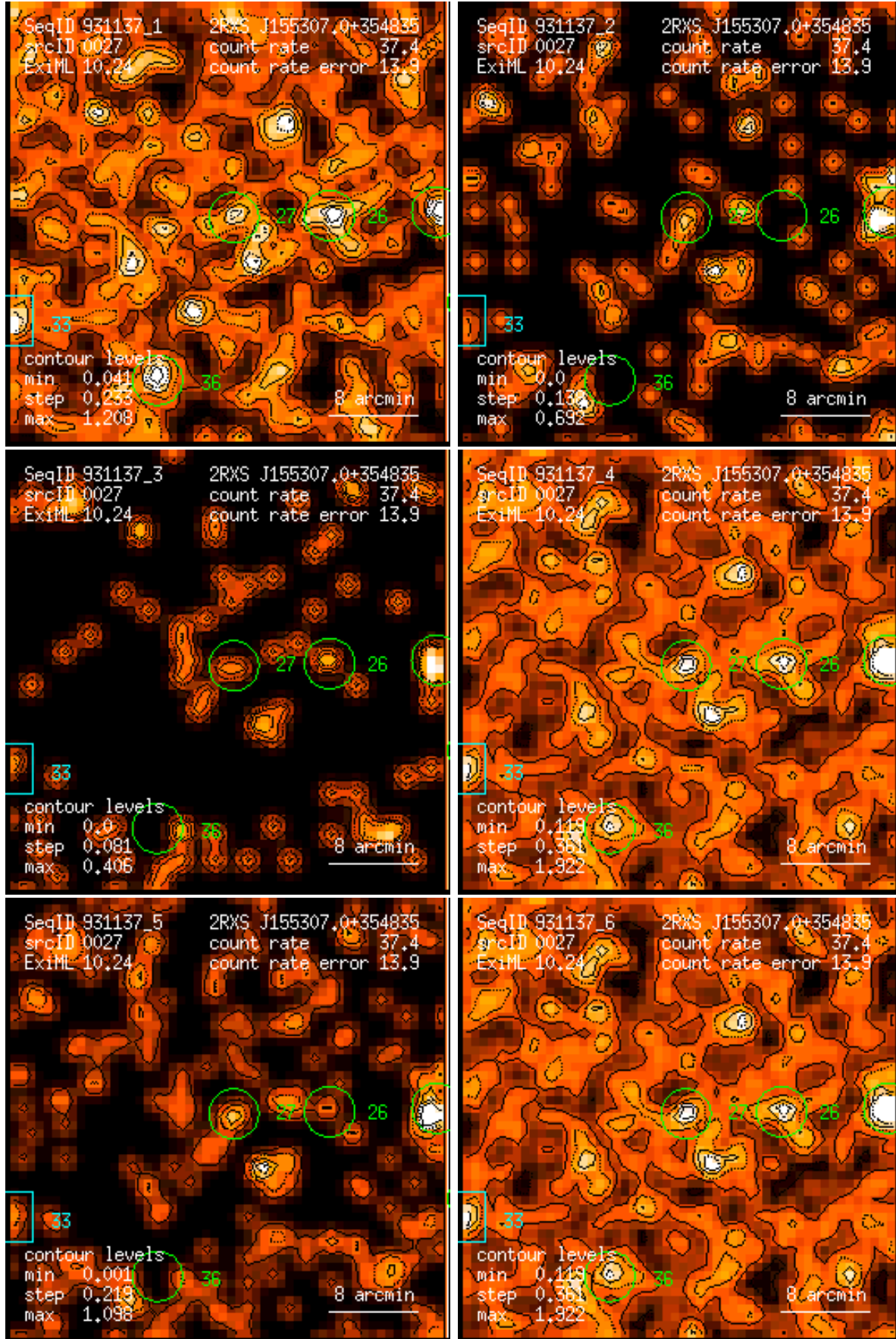
Figure 27: RASS 931137: detection 0027: band rate images, Gaussian filter: (1) PSPC channels 11 – 41, (2) 52 – 90, (3) 91 – 201, (4) 11 – 235, (5) 52 – 201, (6) 11 – 201. Broad band rates in counts/ks. Band rate contour levels in counts/ks/arcmin 2 .
