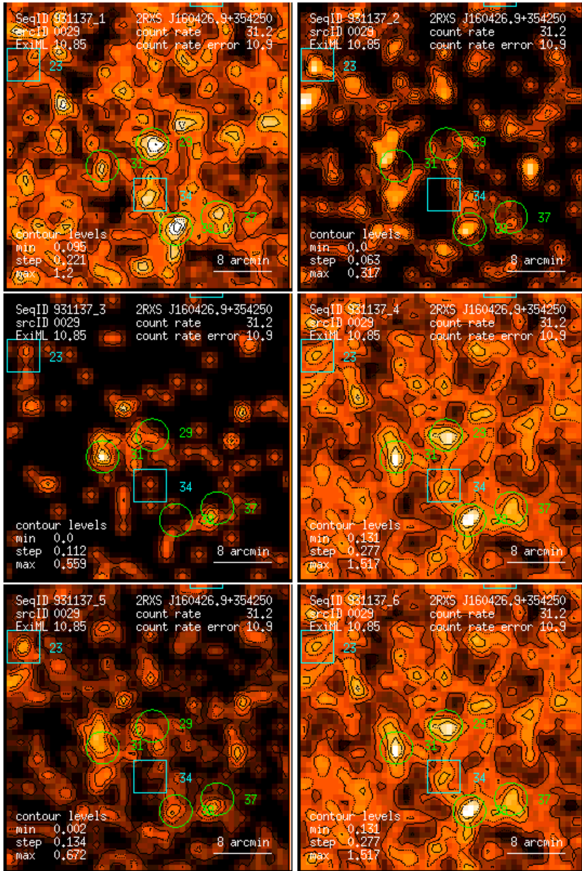
Figure 29: RASS 931137: detection 0029: band rate images, Gaussian filter: (1) PSPC channels 11 – 41, (2) 52 – 90, (3) 91 – 201, (4) 11 – 235, (5) 52 – 201, (6) 11 – 201. Broad band rates in counts/ks. Band rate contour levels in counts/ks/arcmin 2 .
