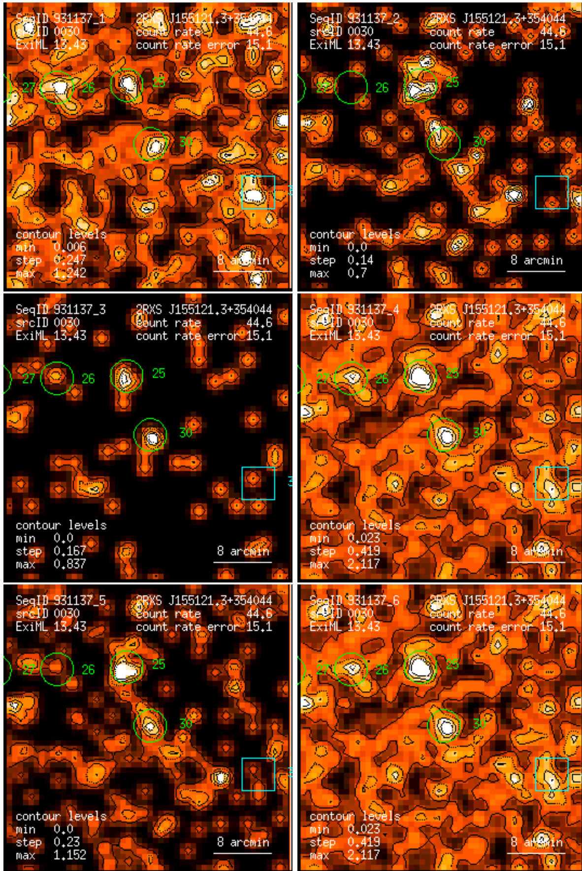
Figure 30: RASS 931137: detection 0030: band rate images, Gaussian filter: (1) PSPC channels 11 – 41, (2) 52 – 90, (3) 91 – 201, (4) 11 – 235, (5) 52 – 201, (6) 11 – 201. Broad band rates in counts/ks. Band rate contour levels in counts/ks/arcmin 2 .
