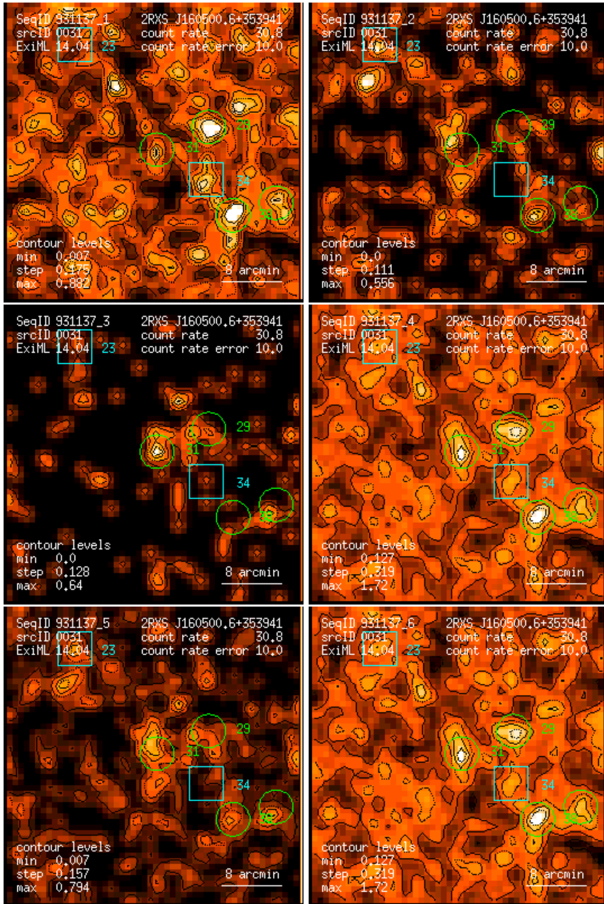
Figure 31: RASS 931137: detection 0031: band rate images, Gaussian filter: (1) PSPC channels 11 – 41, (2) 52 – 90, (3) 91 – 201, (4) 11 – 235, (5) 52 – 201, (6) 11 – 201. Broad band rates in counts/ks. Band rate contour levels in counts/ks/arcmin 2 .
