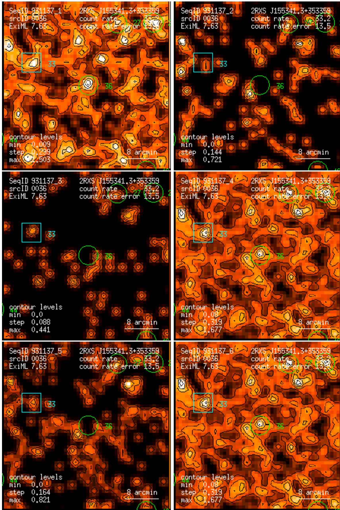
Figure 36: RASS 931137: detection 0036: band rate images, Gaussian filter: (1) PSPC channels 11 – 41, (2) 52 – 90, (3) 91 – 201, (4) 11 – 235, (5) 52 – 201, (6) 11 – 201. Broad band rates in counts/ks. Band rate contour levels in counts/ks/arcmin 2 .
