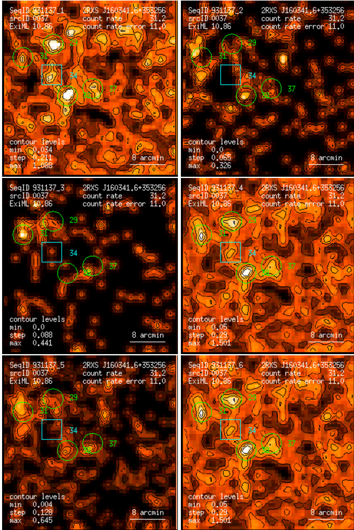
Figure 37: RASS 931137: detection 0037: band rate images, Gaussian filter: (1) PSPC channels 11 – 41, (2) 52 – 90, (3) 91 – 201, (4) 11 – 235, (5) 52 – 201, (6) 11 – 201. Broad band rates in counts/ks. Band rate contour levels in counts/ks/arcmin 2 .
