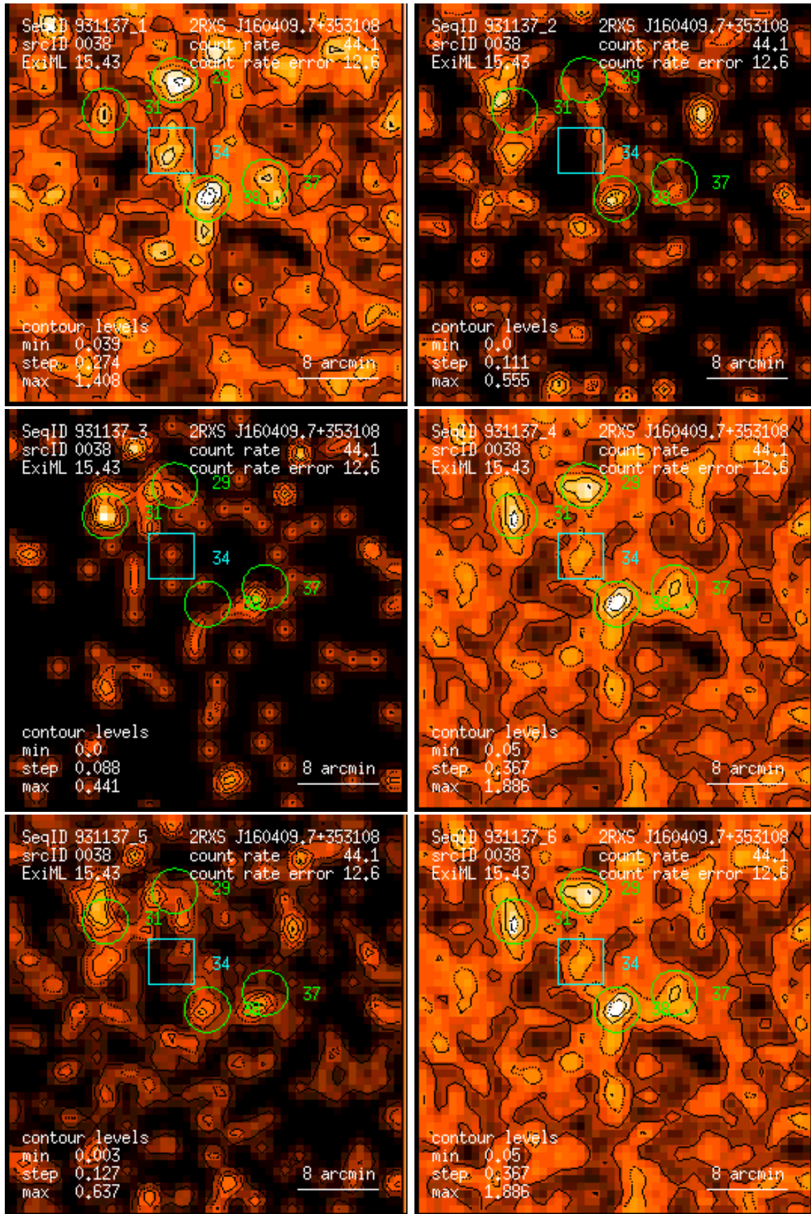
Figure 38: RASS 931137: detection 0038: band rate images, Gaussian filter: (1) PSPC channels 11 – 41, (2) 52 – 90, (3) 91 – 201, (4) 11 – 235, (5) 52 – 201, (6) 11 – 201. Broad band rates in counts/ks. Band rate contour levels in counts/ks/arcmin 2 .
