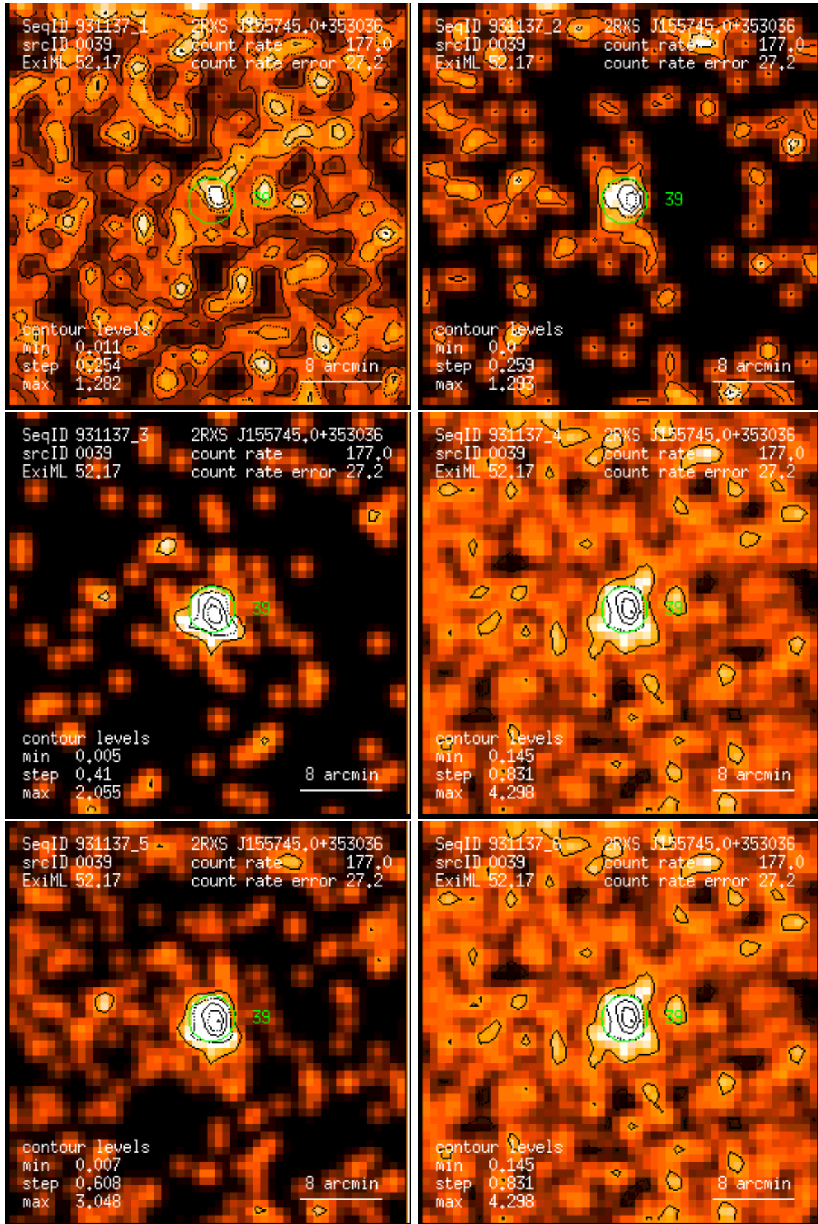
Figure 39: RASS 931137: detection 0039: band rate images, Gaussian filter: (1) PSPC channels 11 – 41, (2) 52 – 90, (3) 91 – 201, (4) 11 – 235, (5) 52 – 201, (6) 11 – 201. Broad band rates in counts/ks. Band rate contour levels in counts/ks/arcmin 2 .
