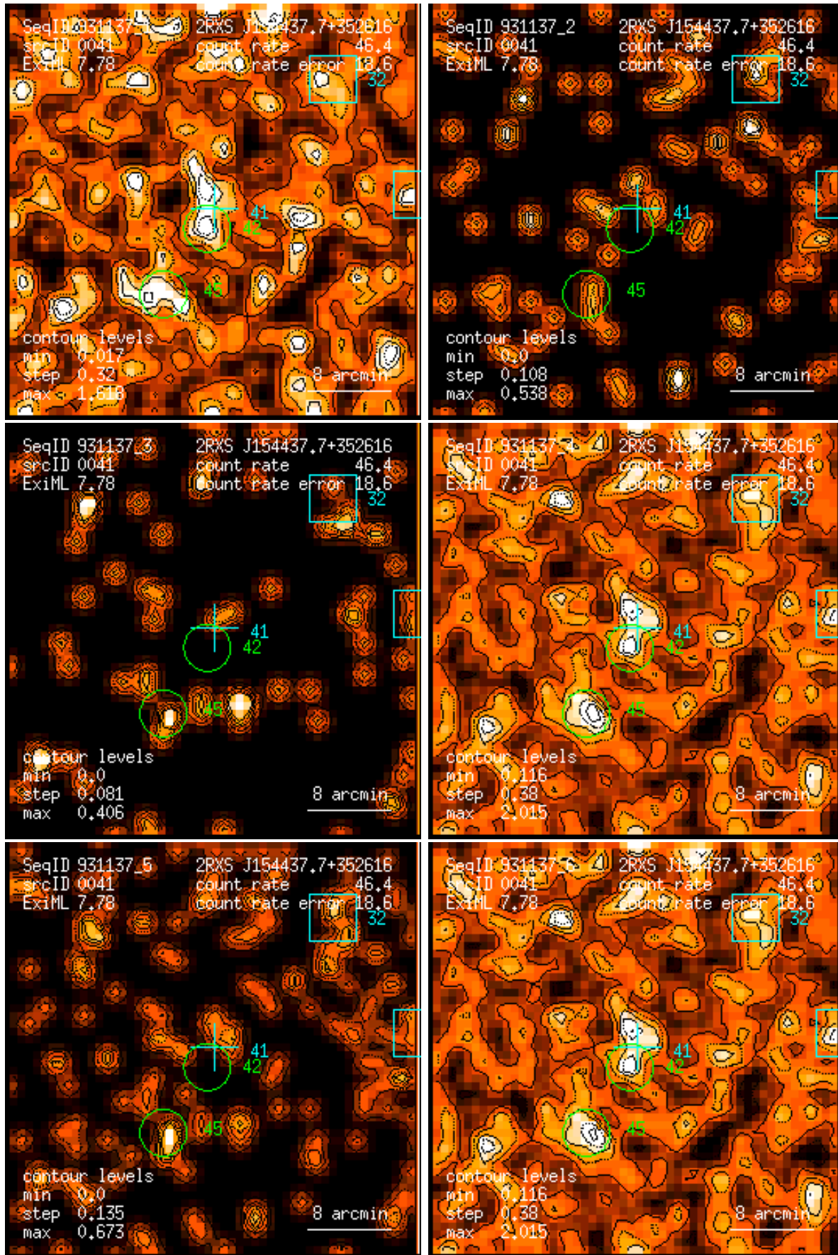
Figure 41: RASS 931137: detection 0041: band rate images, Gaussian filter: (1) PSPC channels 11 – 41, (2) 52 – 90, (3) 91 – 201, (4) 11 – 235, (5) 52 – 201, (6) 11 – 201. Broad band rates in counts/ks. Band rate contour levels in counts/ks/arcmin 2 .
