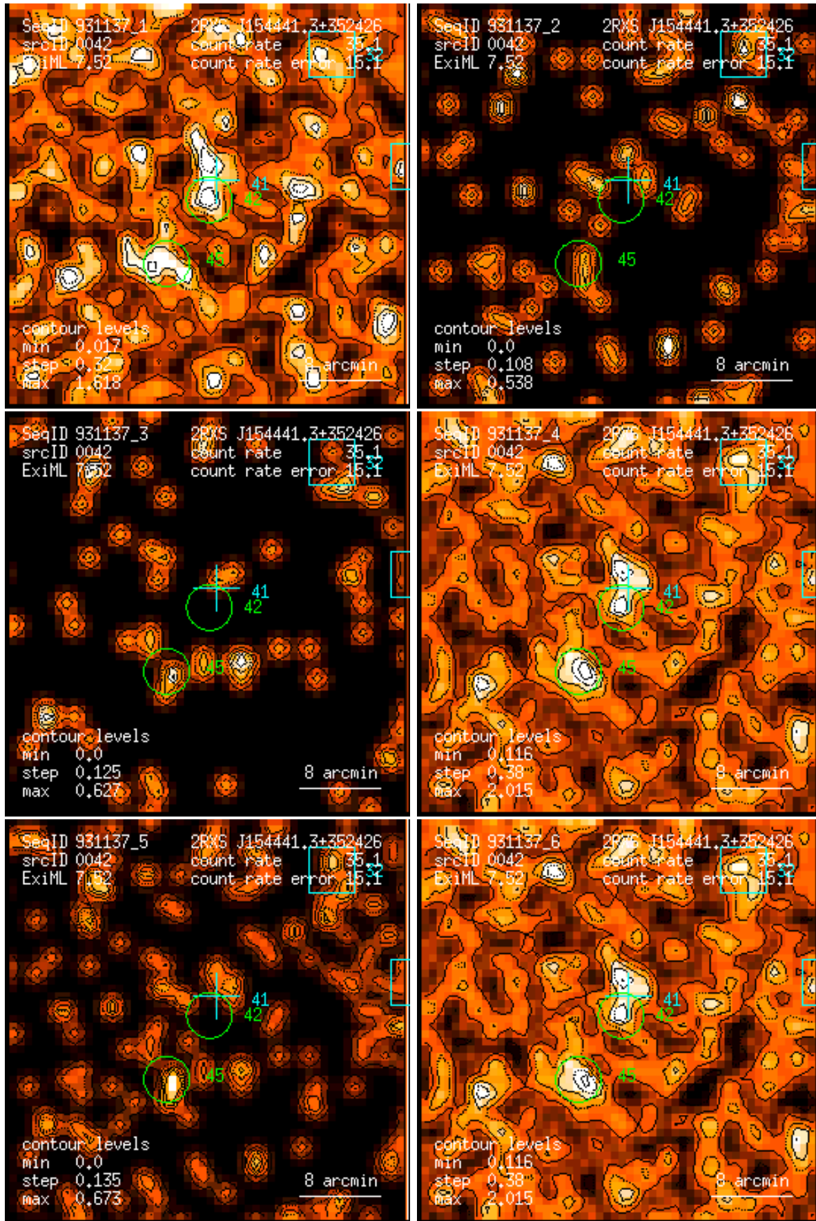
Figure 42: RASS 931137: detection 0042: band rate images, Gaussian filter: (1) PSPC channels 11 – 41, (2) 52 – 90, (3) 91 – 201, (4) 11 – 235, (5) 52 – 201, (6) 11 – 201. Broad band rates in counts/ks. Band rate contour levels in counts/ks/arcmin 2 .
