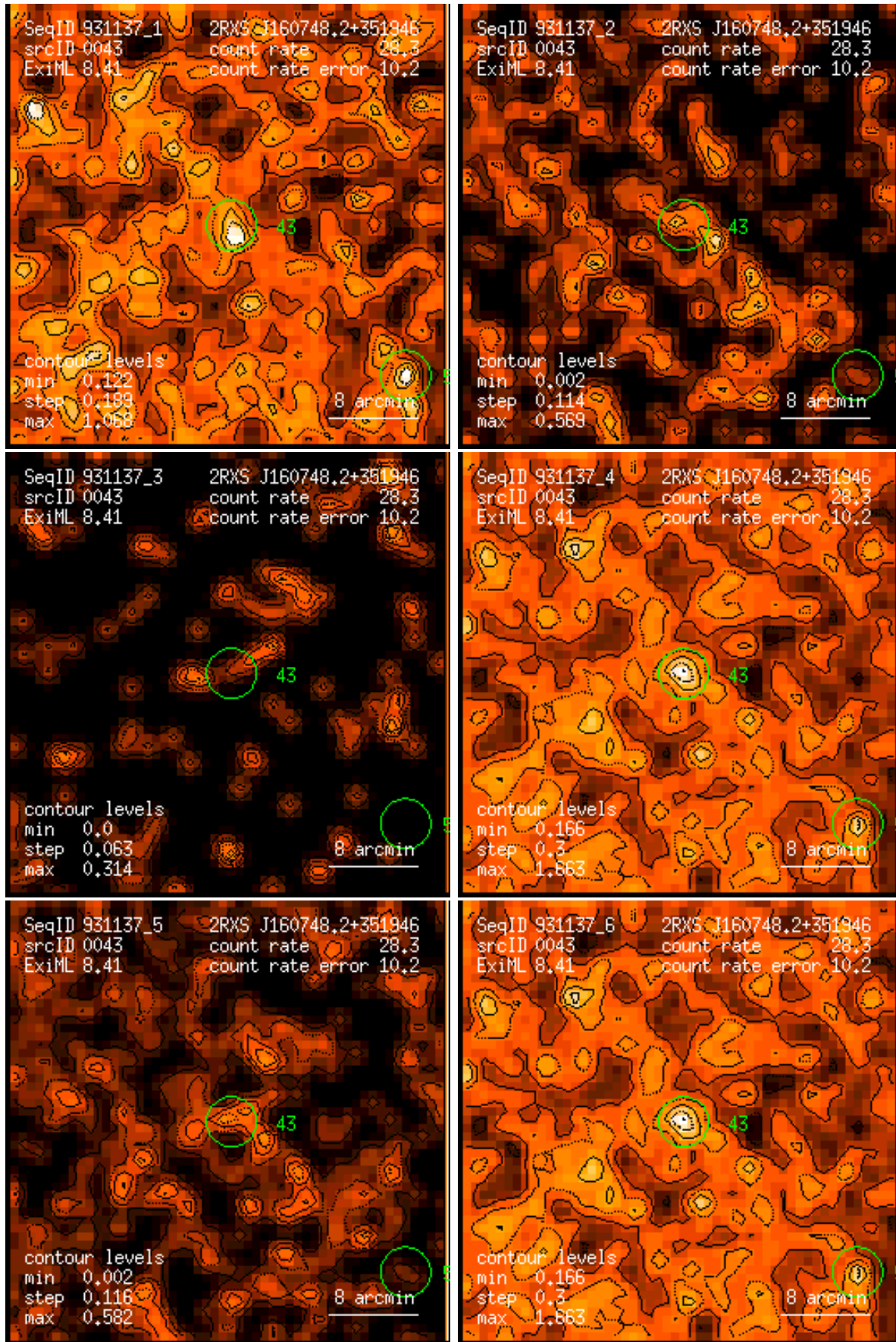
Figure 43: RASS 931137: detection 0043: band rate images, Gaussian filter: (1) PSPC channels 11 – 41, (2) 52 – 90, (3) 91 – 201, (4) 11 – 235, (5) 52 – 201, (6) 11 – 201. Broad band rates in counts/ks. Band rate contour levels in counts/ks/arcmin 2 .
