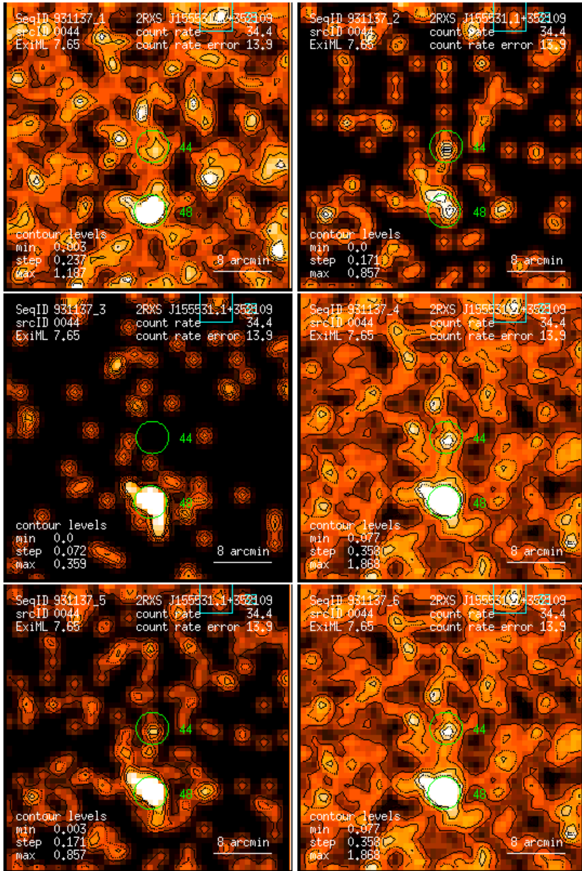
Figure 44: RASS 931137: detection 0044: band rate images, Gaussian filter: (1) PSPC channels 11 – 41, (2) 52 – 90, (3) 91 – 201, (4) 11 – 235, (5) 52 – 201, (6) 11 – 201. Broad band rates in counts/ks. Band rate contour levels in counts/ks/arcmin 2 .
