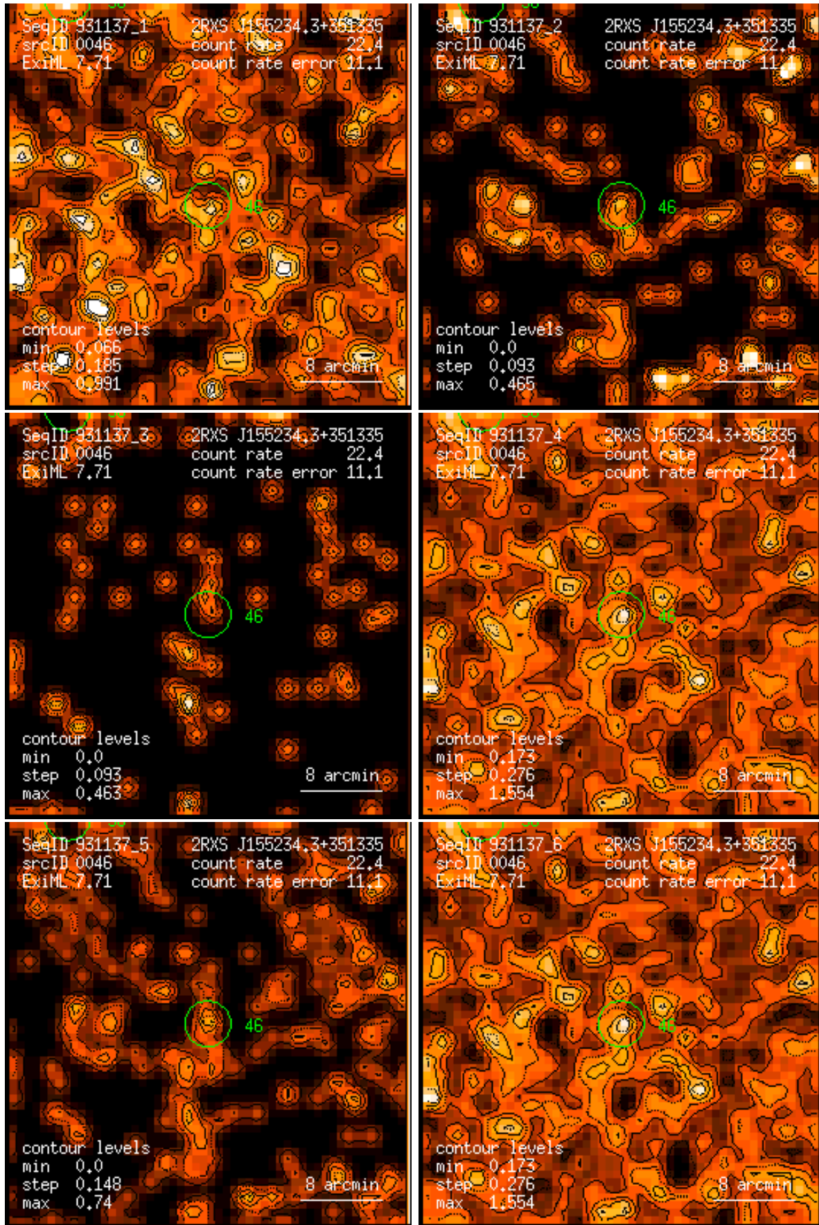
Figure 46: RASS 931137: detection 0046: band rate images, Gaussian filter: (1) PSPC channels 11 – 41, (2) 52 – 90, (3) 91 – 201, (4) 11 – 235, (5) 52 – 201, (6) 11 – 201. Broad band rates in counts/ks. Band rate contour levels in counts/ks/arcmin 2 .
