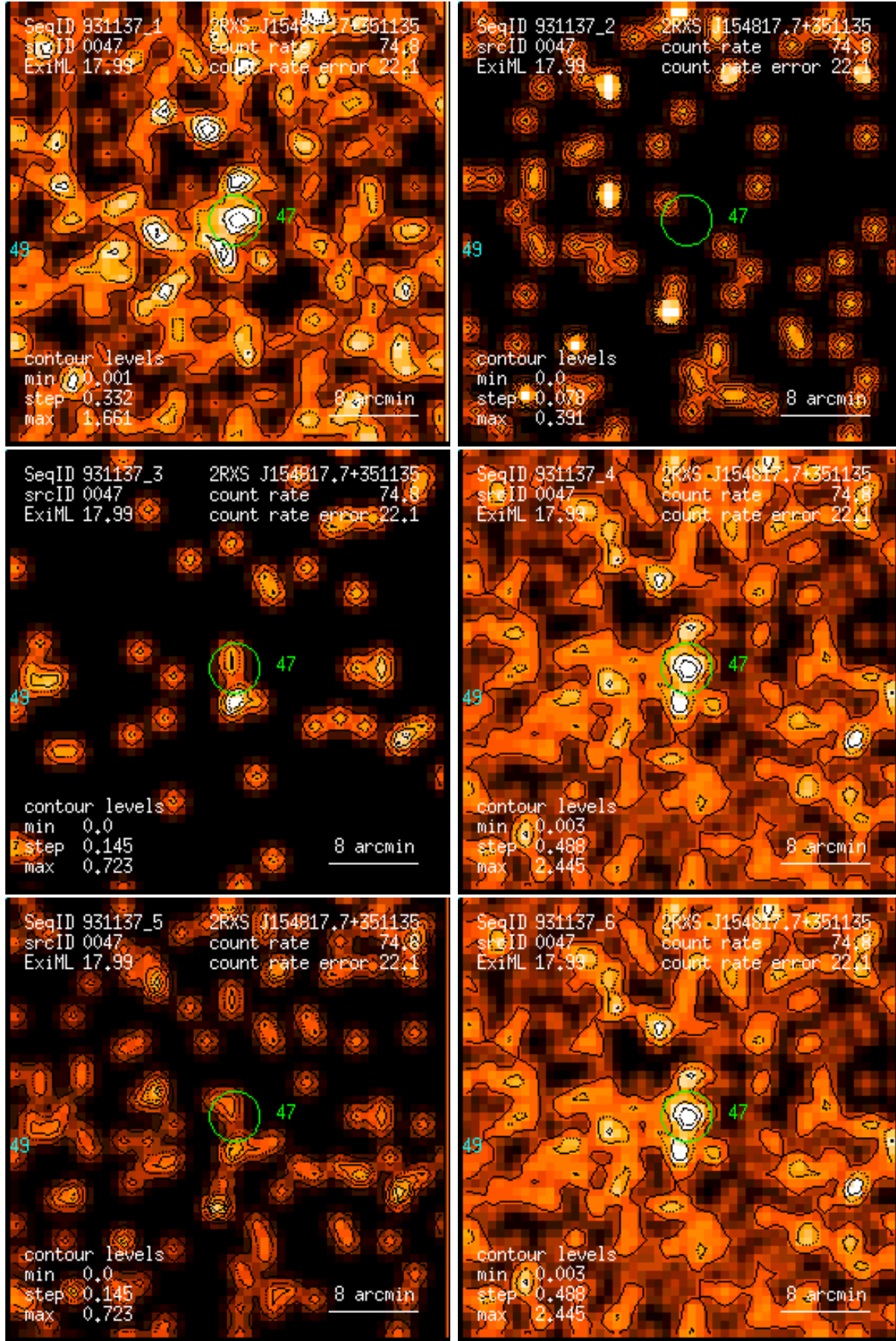
Figure 47: RASS 931137: detection 0047: band rate images, Gaussian filter: (1) PSPC channels 11 – 41, (2) 52 – 90, (3) 91 – 201, (4) 11 – 235, (5) 52 – 201, (6) 11 – 201. Broad band rates in counts/ks. Band rate contour levels in counts/ks/arcmin 2 .
