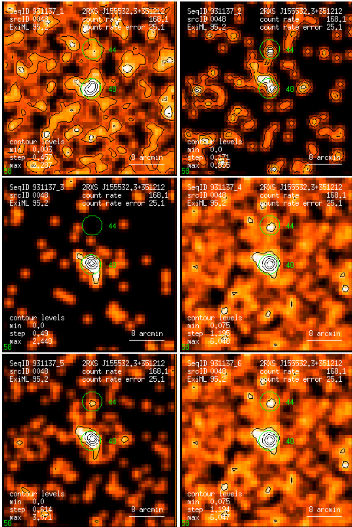
Figure 48: RASS 931137: detection 0048: band rate images, Gaussian filter: (1) PSPC channels 11 – 41, (2) 52 – 90, (3) 91 – 201, (4) 11 – 235, (5) 52 – 201, (6) 11 – 201. Broad band rates in counts/ks. Band rate contour levels in counts/ks/arcmin 2 .
