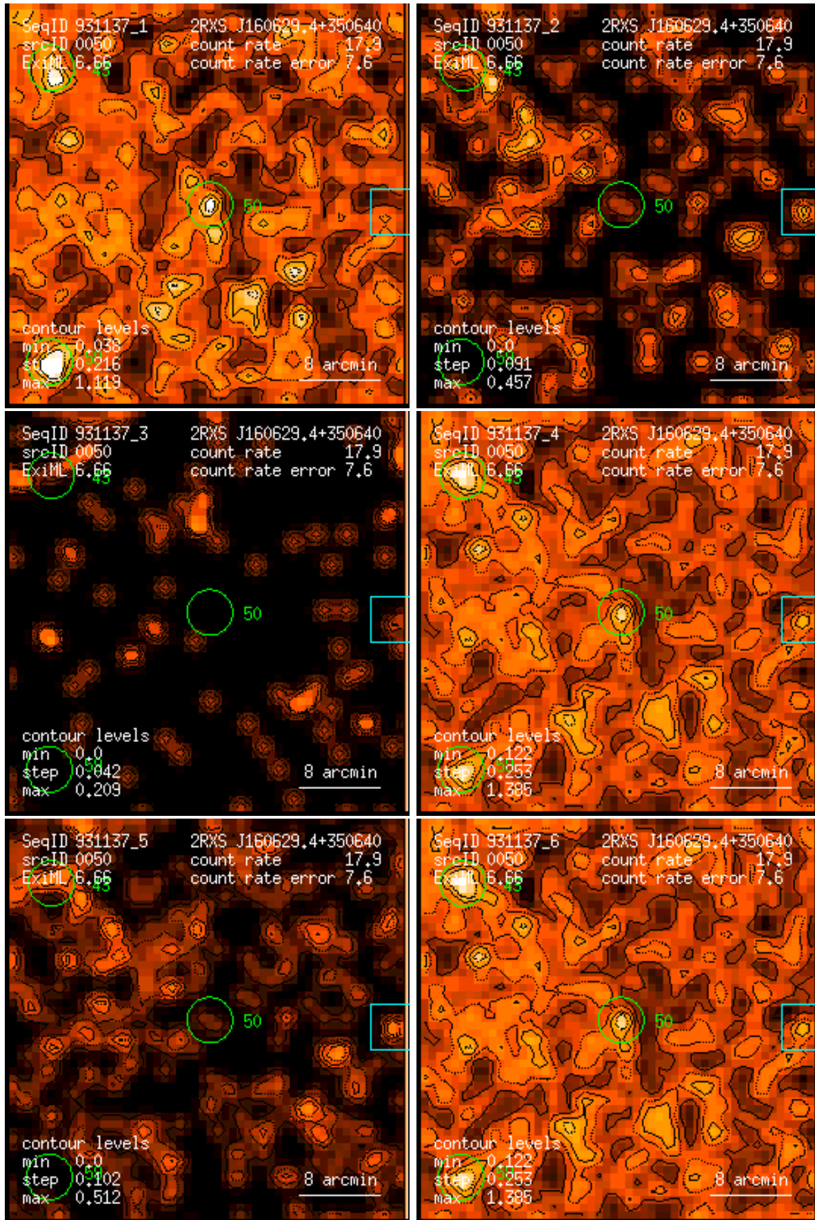
Figure 50: RASS 931137: detection 0050: band rate images, Gaussian filter: (1) PSPC channels 11 – 41, (2) 52 – 90, (3) 91 – 201, (4) 11 – 235, (5) 52 – 201, (6) 11 – 201. Broad band rates in counts/ks. Band rate contour levels in counts/ks/arcmin 2 .
