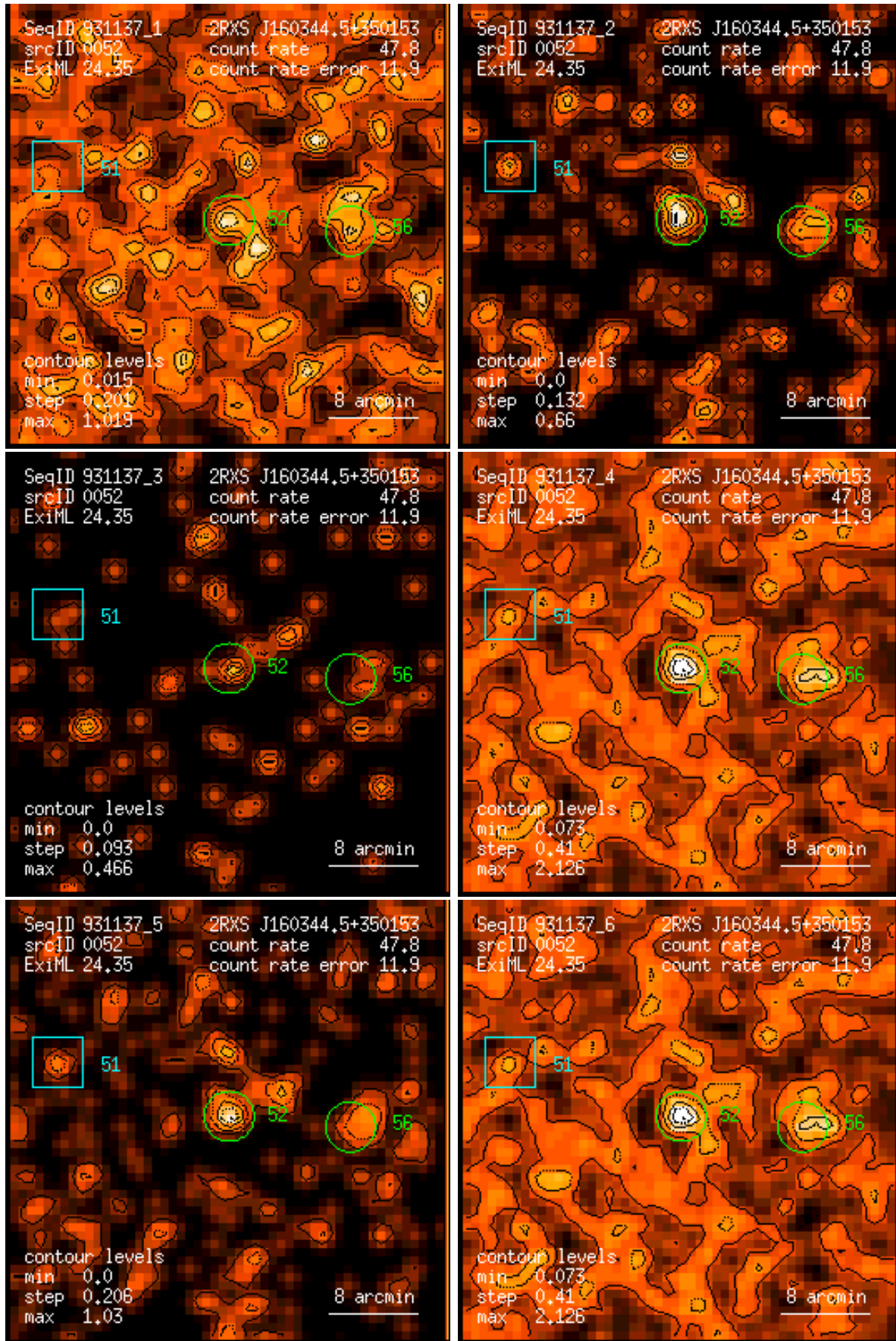
Figure 52: RASS 931137: detection 0052: band rate images, Gaussian filter: (1) PSPC channels 11 – 41, (2) 52 – 90, (3) 91 – 201, (4) 11 – 235, (5) 52 – 201, (6) 11 – 201. Broad band rates in counts/ks. Band rate contour levels in counts/ks/arcmin 2 .
